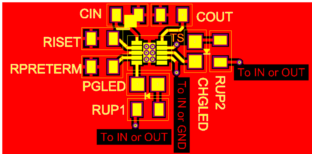
图 11-1. Board Layout
