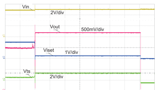
图 9-10. Battery Removal - GND Removed 1st, 42 \Omega Load
