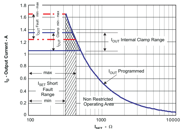
图 8-5. Programmed/Clamped Out Current (BQ24040)
