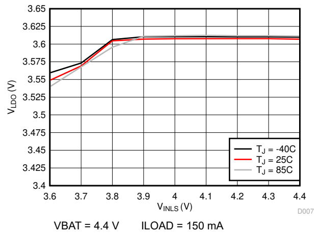
图 8-12. LDO Line Regulation (VLDO = 3.6 V)
