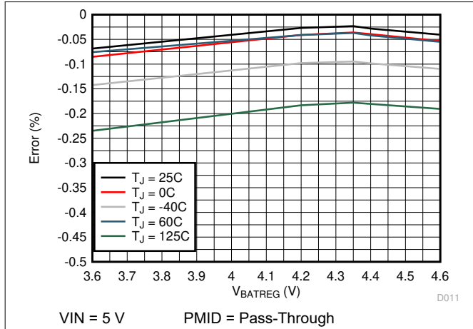
图 8-1. Battery Regulation Voltage Accuracy vs. VBATREG Setting
