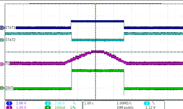
图 8-13. TS Change Response
