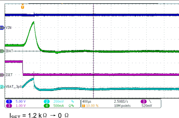
图 8-11. ISET Short-Circuit Response
