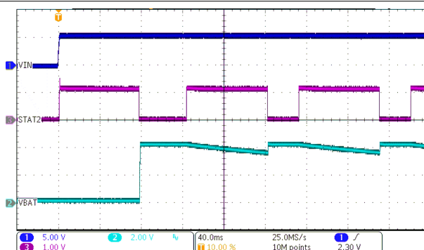
图 8-3. Power Up without Battery
