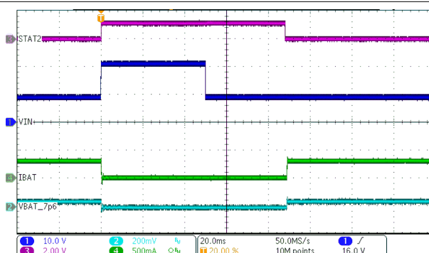
图 8-7. IN OVP Response
