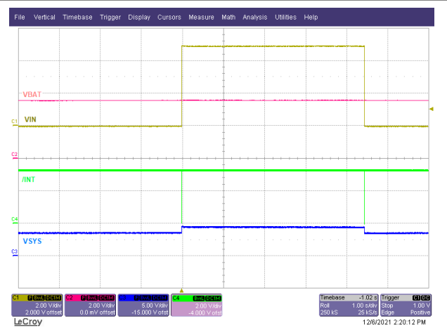
图 9-11. Power Good Interrupt on /INT
