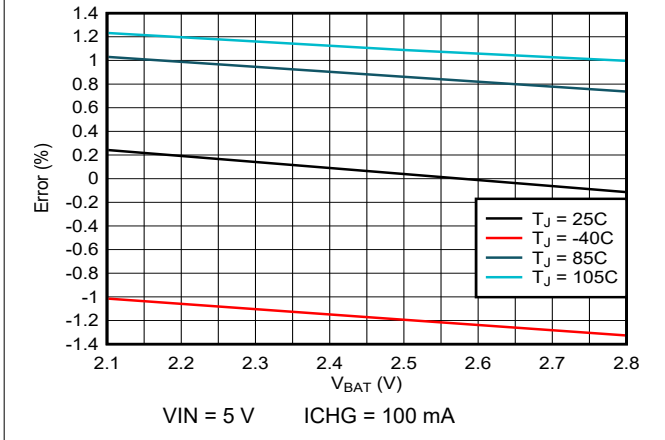
图 7-3. Precharge Accuracy vs Battery Voltage
