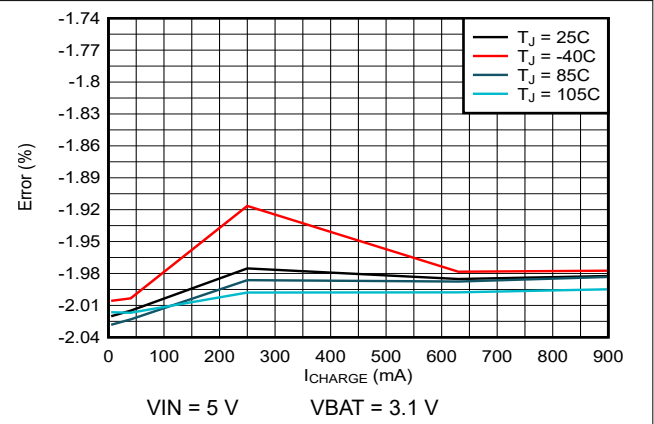
图 7-2. Charge Current Accuracy vs. ICHARGE Setting
