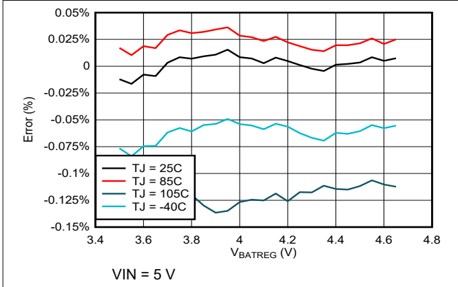
图 7-1. Battery Regulation Voltage Accuracy vs. VBATREG Setting
