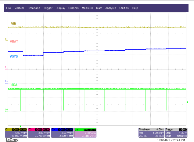
图 9-13. SYS Regulation Sweep
