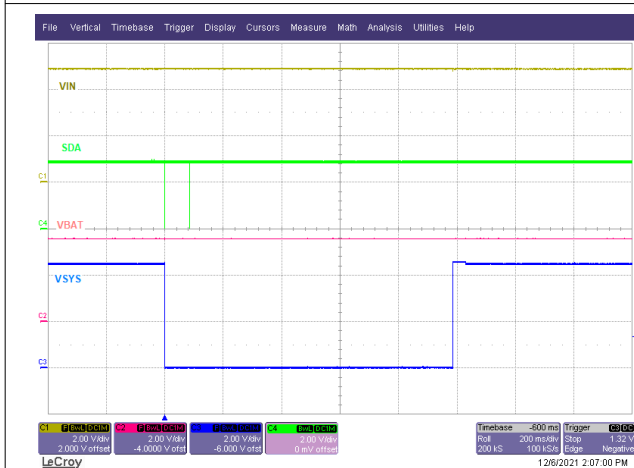
图 9-8. Hardware Reset Through I 2 C
