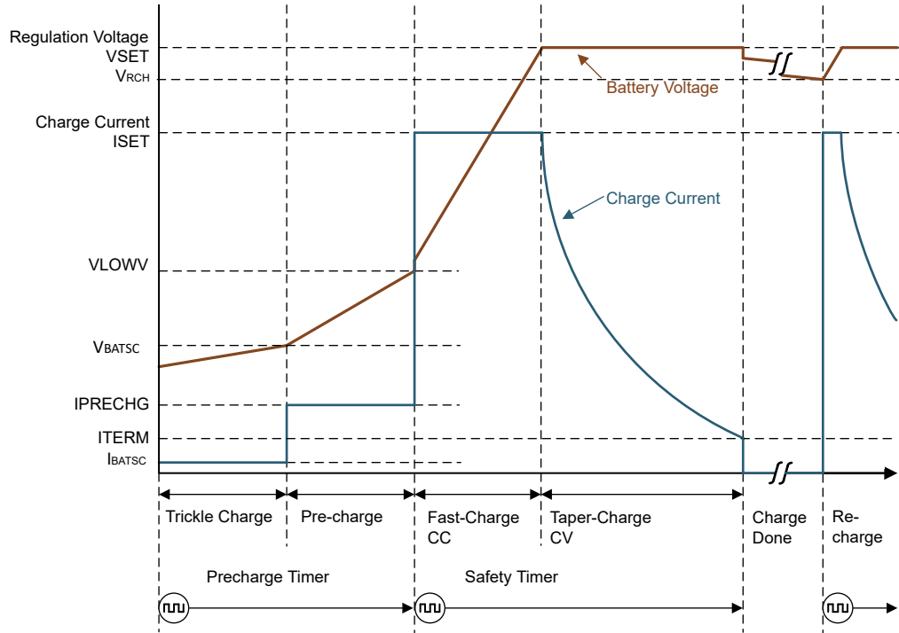
图 8-2. Typical Charging Profile of a Battery
