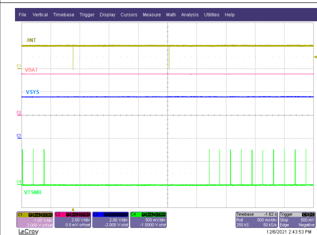
图 9-17. Long Press Interrupt with VIN Present
