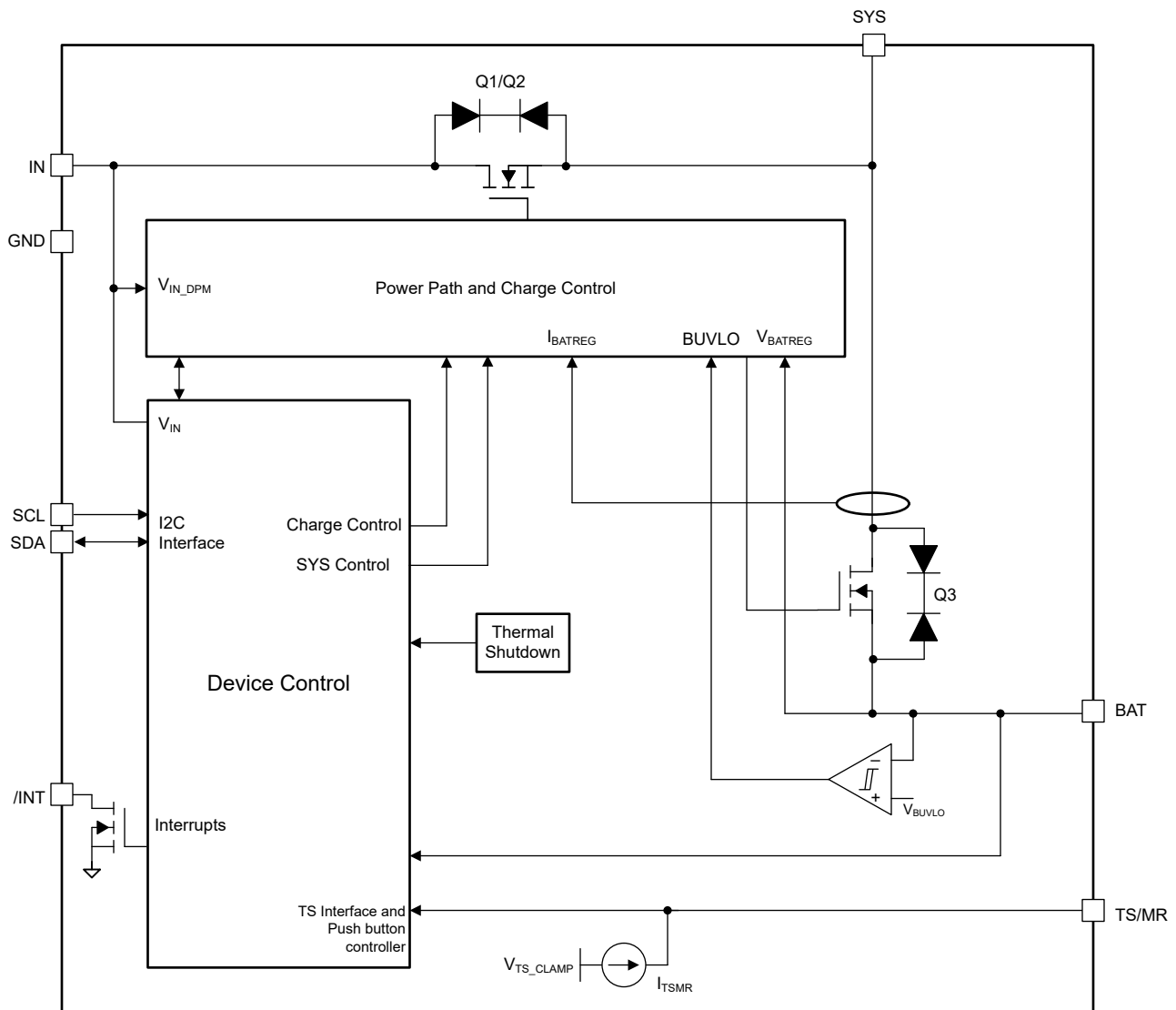
图 8-3. Functional Block Diagram
