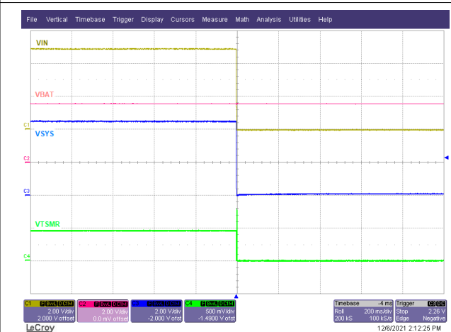
图 9-7. Enter Shipmode with Push Button Long Press
