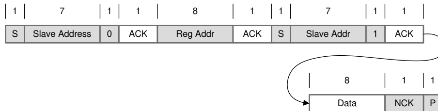
图 9-17. Single Read
