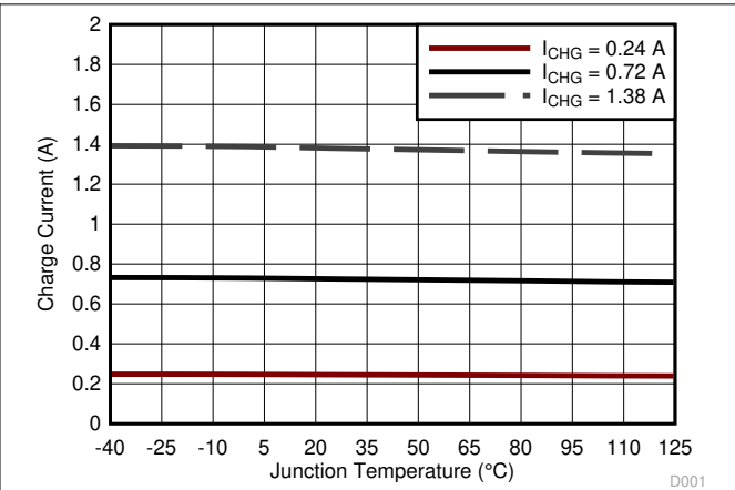
图 8-8. Charge Current vs. Junction Temperature
