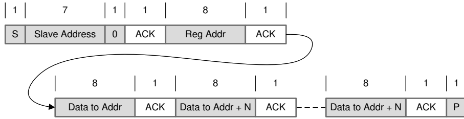
图 9-18. Multi-Write
