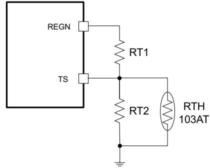
图 9-5. TS Resistor Network
