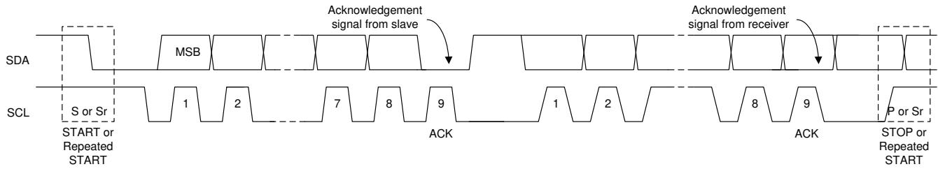
图 9-14. Data Transfer on the I 2 C Bus
