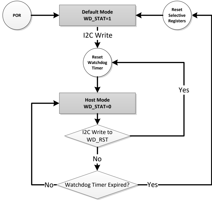
图 7-8. Watchdog Timer Flow Chart
