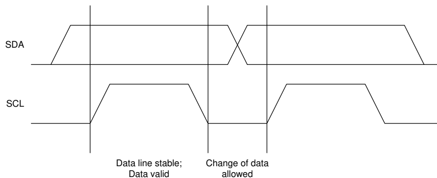
图 7-9. Bit Transfer on the I 2 C Bus
