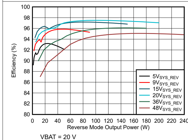
VBAT = 20 V 图 7-9. Reverse Mode Efficiency (5s battery configuration)
