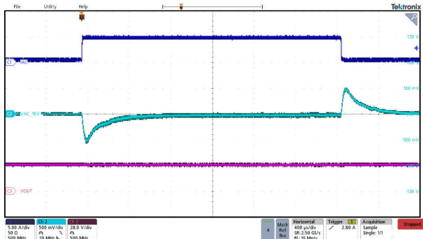
图 9-17. Reverse Mode Buck-Boost Transient Response
