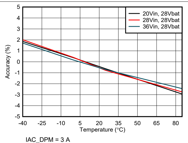
IAC_DPM = 3 A 图 7-8. Input Current (IAC_DPM) Regulation Accuracy vs Temperature
