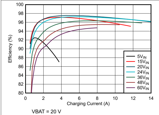
图 7-1. Charge Efficiency vs Charge Current (5s battery configuration)
