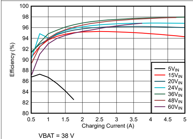
图 7-3. Charge Efficiency vs Charge Current (10s battery configuration)
