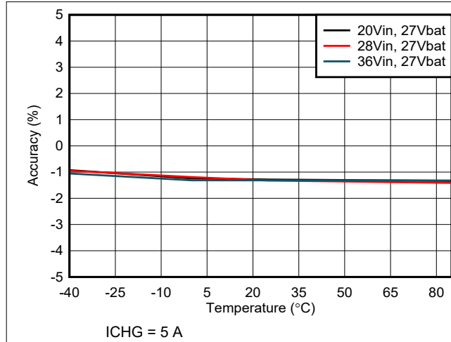
ICHG = 5 A 图 7-5. Charge Current Accuracy vs Temperature
