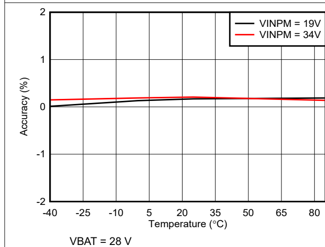
VBAT = 28 V 图 7-7. Input Voltage (VAC_DPM) Regulation Accuracy vs Temperature
