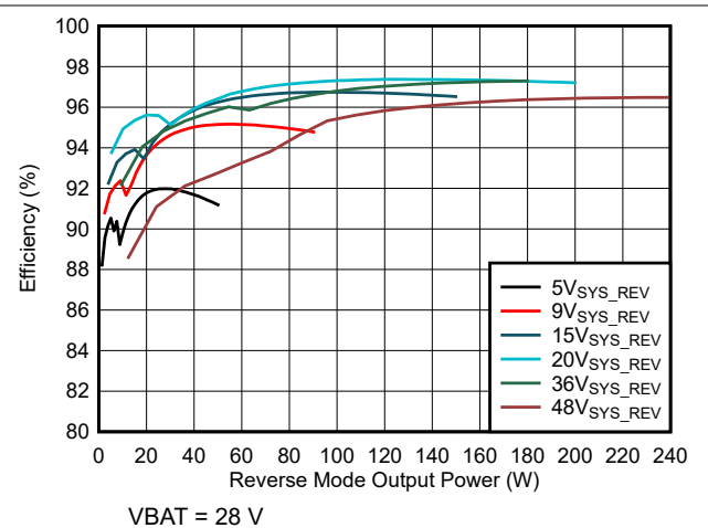
VBAT = 28 V 图 7-10. Reverse Mode Efficiency (7s battery configuration)
