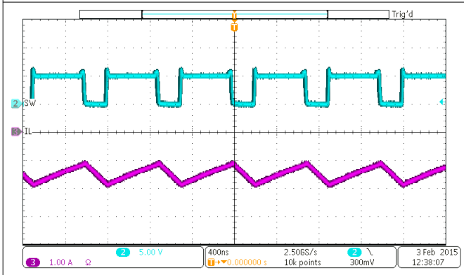
VBAT = 3.8 V I LOAD = 1 A 图 10-10. Boost Mode Switching Waveform
