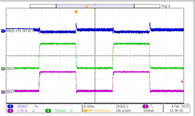
VBAT = 3.8 V I LOAD = 0 A - 1 A 图 10-11. Boost Mode Load Transient
