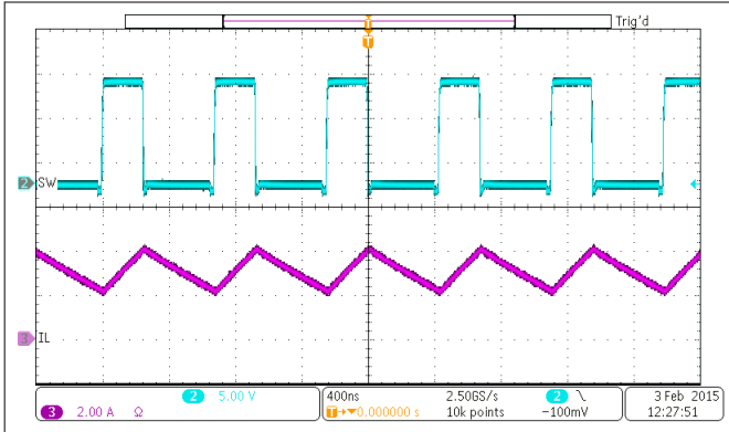
VBUS = 12 V VBAT = 3.8 V ICHG = 3 A 图 10-8. PWM Switching Waveform
