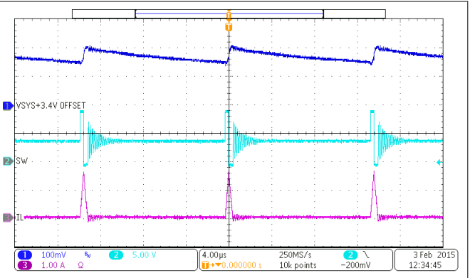
VBUS = 9V I SYS = 10 mA, Charge Disable No Battery 图 10-9. PFM Switching Waveform
