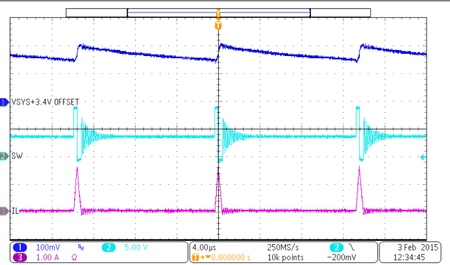
图 9-9. Load Transient During Supplement Mode
