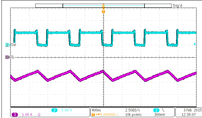
图 9-12. Boost Mode Switching Waveform
