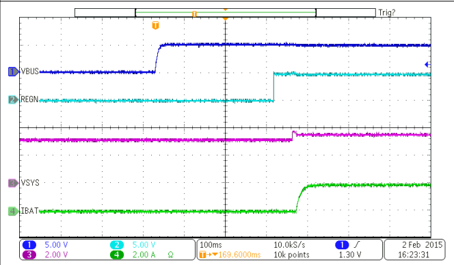
图 9-5. Power Up with Charge Enabled
