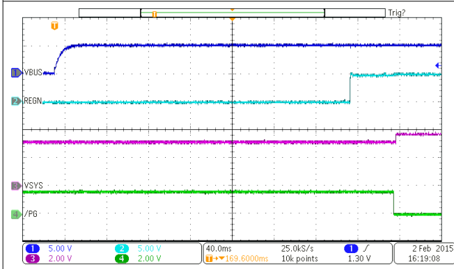
图 9-2. Power Up from USB100
