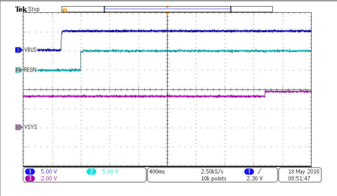
图 9-3. Power Up with Charge Disabled
