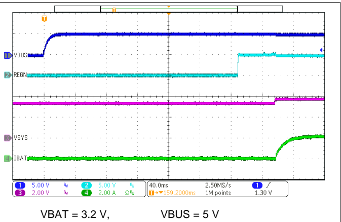
图 42. Power Up with Charge Enabled
