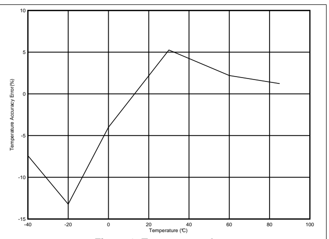
Figure 8. Temperature Accuracy
