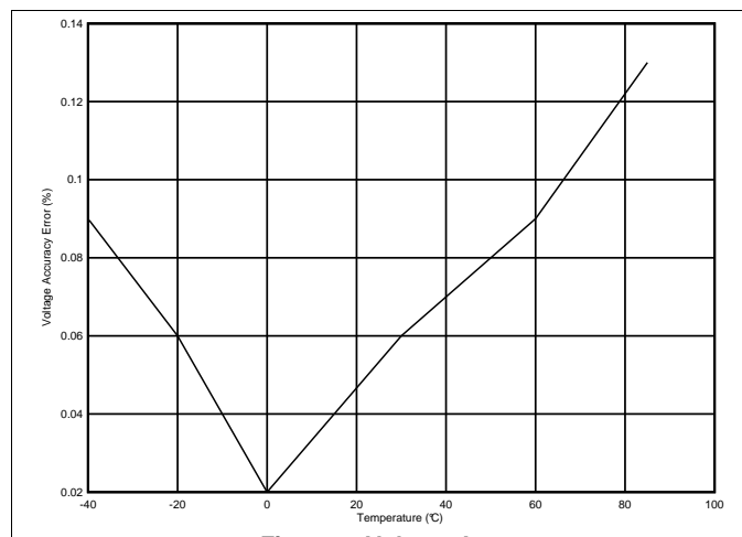
Figure 7. Voltage Accuracy
