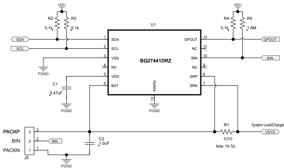
Figure 6. Typical Application
