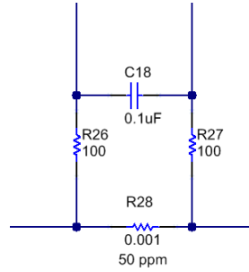
图 9-6. Differential Filter
