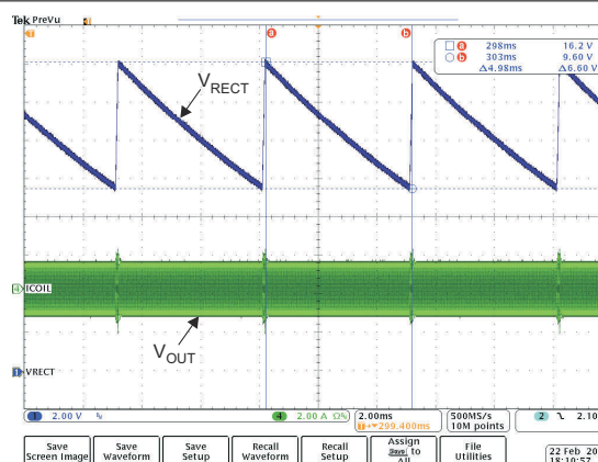
图 8-12. Rectifier Overvoltage Clamp ( f_{op} = 110 \text{ kHz} )
