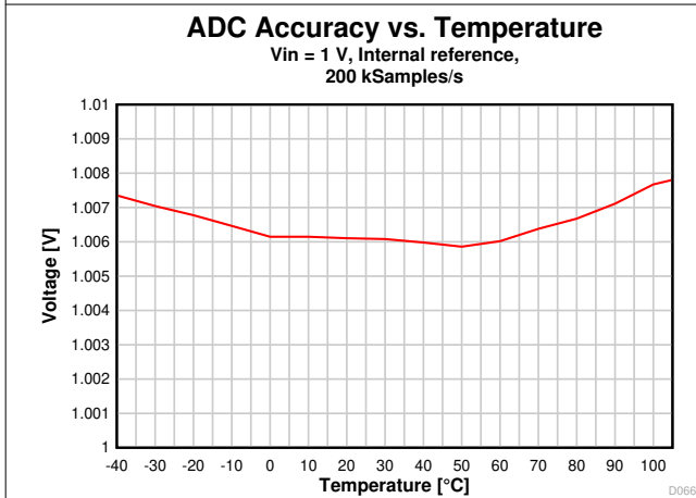
图 8-32. ADC Accuracy vs. Temperature
