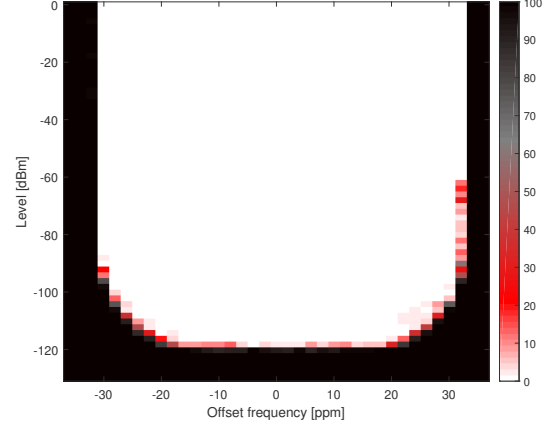
8-18. PER vs. Level vs. Frequency (SimpleLink™ Long Range 5 kbps, 868 MHz)
