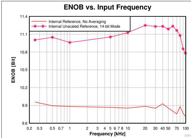
图 8-28. ENOB vs. Input Frequency
