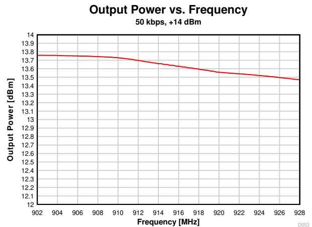
图 8-26. Output Power vs. Frequency (50 kbps, 915 MHz)
