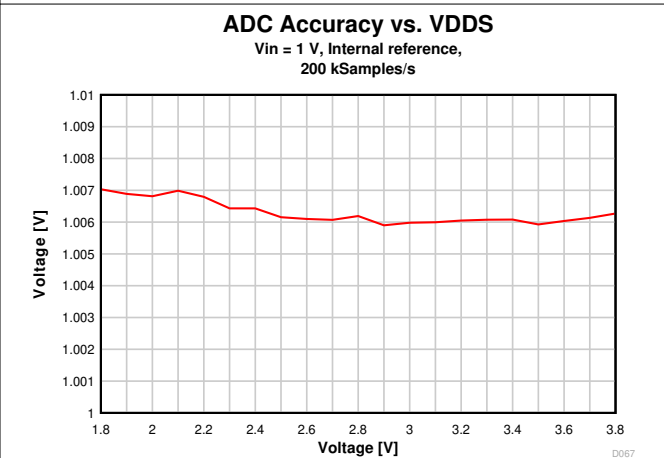
图 8-33. ADC Accuracy vs. Supply Voltage (VDDS)
