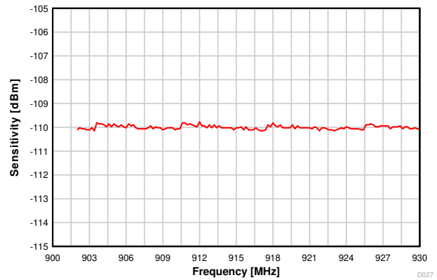
8-14. Sensitivity vs. Frequency (50 kbps, 915 MHz)
