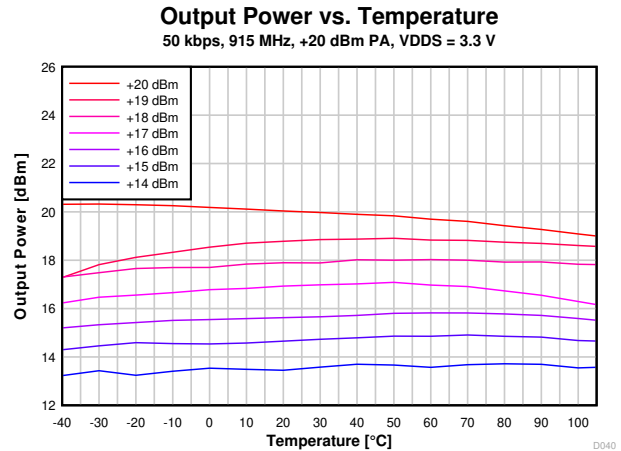
图 8-22. Output Power vs. Temperature (50 kbps, 915 MHz)
