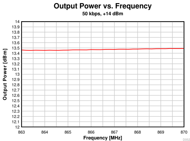
图 8-25. Output Power vs. Frequency (50 kbps, 868 MHz)
