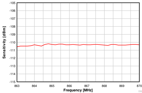
8-13. Sensitivity vs. Frequency (50 kbps, 868 MHz)
