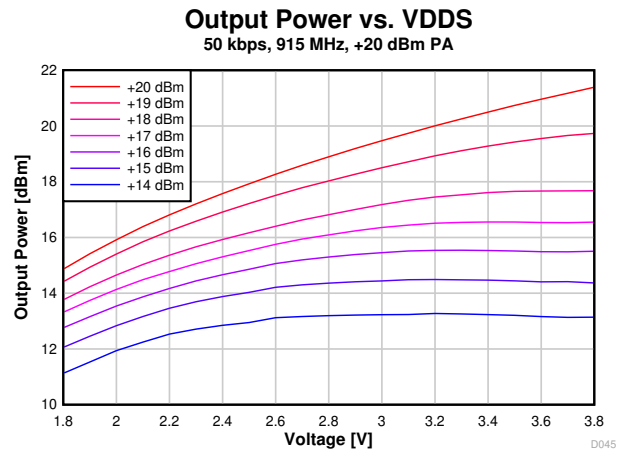
图 8-24. Output Power vs. Supply Voltage (VDD5) (50 kbps, 915 MHz)
