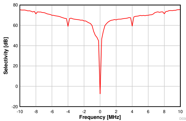
8-17. Selectivity vs. Frequency Offset (50 kbps, 868.3 MHz)
