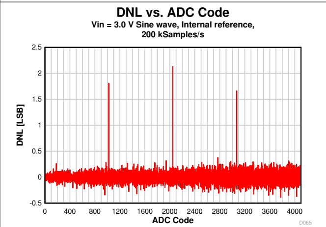
图 8-31. DNL vs. ADC Code
