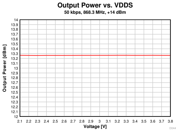
图 8-23. Output Power vs. Supply Voltage (VDD5) (50 kbps, 868.3 MHz)
