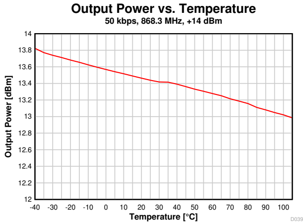
图 8-21. Output Power vs. Temperature (50 kbps, 868.3 MHz)
