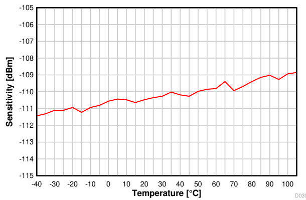
8-15. Sensitivity vs. Temperature (50 kbps, 868.3 MHz)
