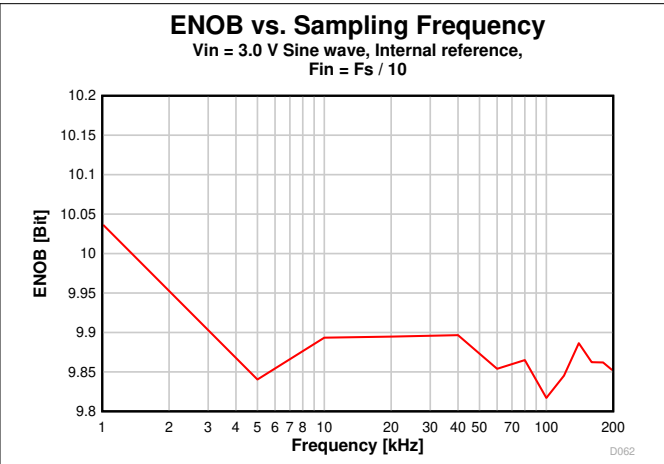
图 8-29. ENOB vs. Sampling Frequency
