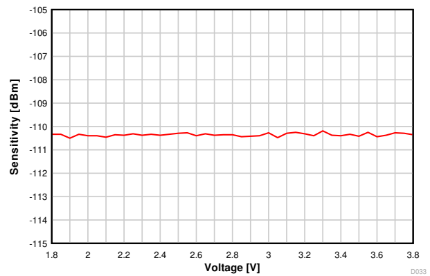
8-16. Sensitivity vs. Supply Voltage (VDD5) (50 kbps, 868.3 MHz)
