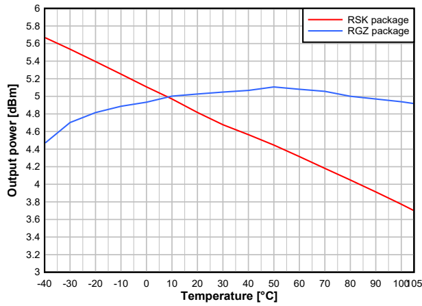
图 8-27. Output Power vs. Temperature (BLE 1 Mbps, 2.44 GHz, +5 dBm)
