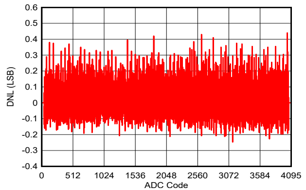
图 7-30. DNL vs. ADC Code ( V_{in}= 3V Sine Wave, Internal Reference, 200 kps)
