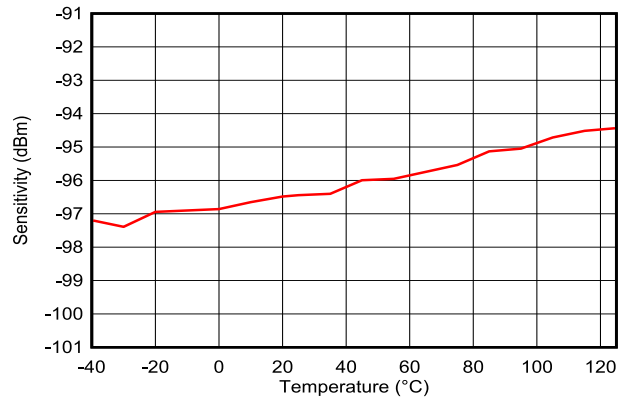
图 7-15. Sensitivity vs. Temperature (BLE 1 Mbps, 2.44 GHz)
