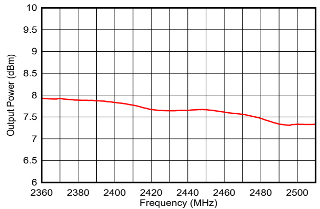
图 7-24. Output Power vs. Frequency (BLE 1 Mbps, +8 dBm)
