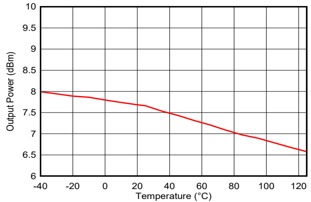
图 7-20. Output Power vs. Temperature (BLE 1 Mbps, 2.44 GHz, +8 dBm)
