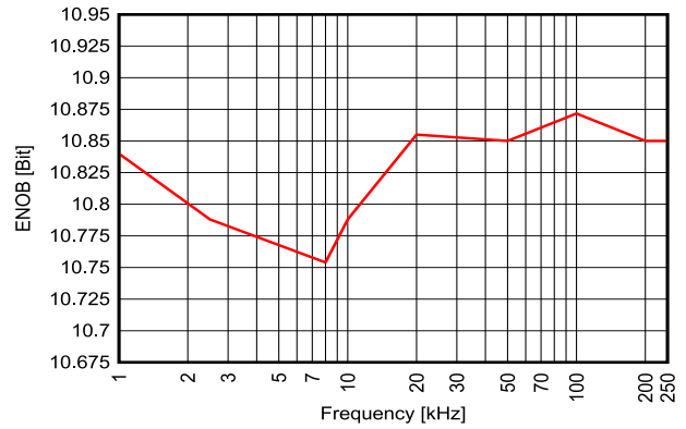
图 7-26. ENOB vs. Sampling Frequency ( V_{in}= 3V Sine Wave, Internal Reference, F_{in}=F_s/10 )
