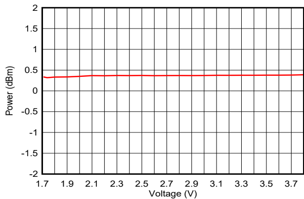
图 7-21. Output Power vs. Supply Voltage (VDD5) (BLE 1 Mbps, 2.44 GHz, 0 dBm)
