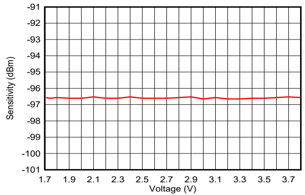
图 7-17. Sensitivity vs. Supply Voltage (VDD5) (BLE 1 Mbps, 2.44 GHz, DCDC Off)
