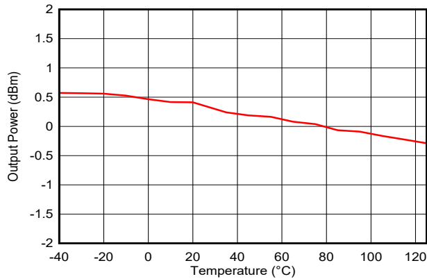
图 7-19. Output Power vs. Temperature (BLE 1 Mbps, 2.44 GHz, 0 dBm)
