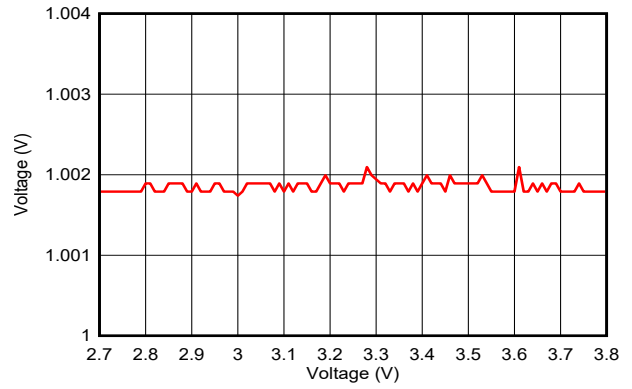
图 7-32. ADC Accuracy vs. Supply Voltage ( V_{in}=1V , Internal Reference, 200 kps)
