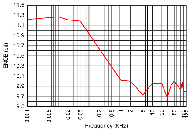
图 7-27. ENOB vs. Input Frequency (External Reference = 3.0 V)
