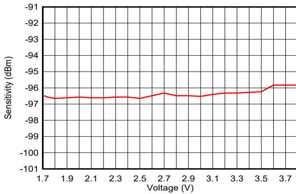
图 7-16. Sensitivity vs. Supply Voltage (VDD5) (BLE 1 Mbps, 2.44 GHz)
