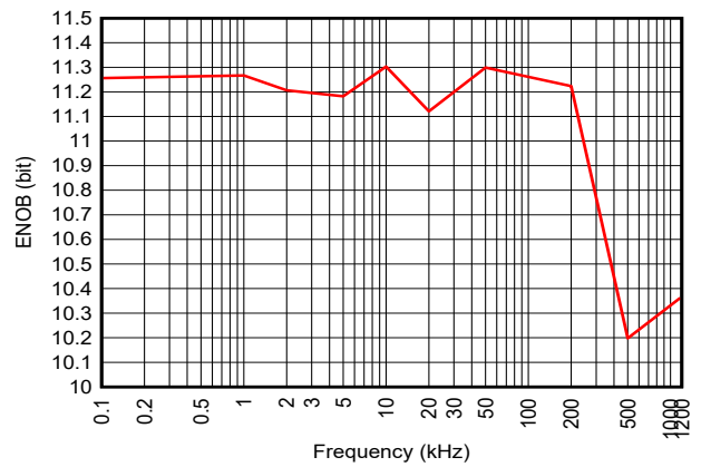
图 7-28. ENOB vs. Sampling Frequency ( V_{in}= 3V Sine Wave, External Reference = 3.0 V, F_{in}=F_s/10 )
