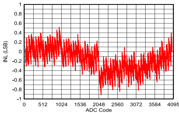
图 7-29. INL vs. ADC Code ( V_{in}= 3V Sine Wave, Internal Reference, 200 kps)
