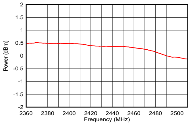
图 7-23. Output Power vs. Frequency (BLE 1 Mbps, 0 dBm)
