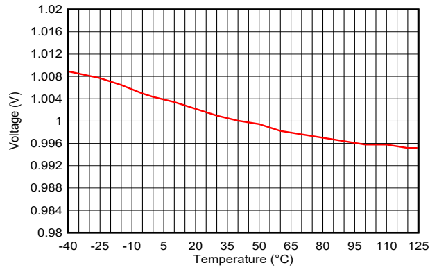
图 7-31. ADC Accuracy vs. Temperature ( V_{in}=1V , Internal Reference, 200 kps)
