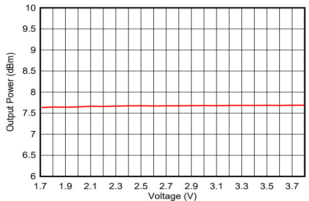
图 7-22. Output Power vs. Supply Voltage (VDD5) (BLE 1 Mbps, 2.44 GHz, +8 dBm)
