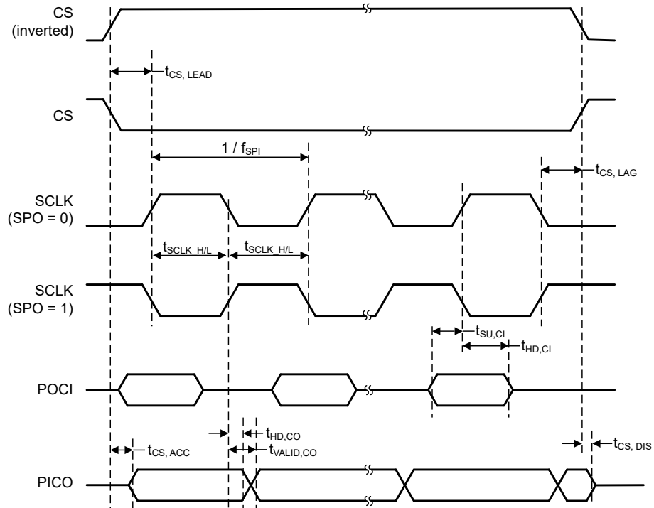
Controller Mode, SPH = 0
