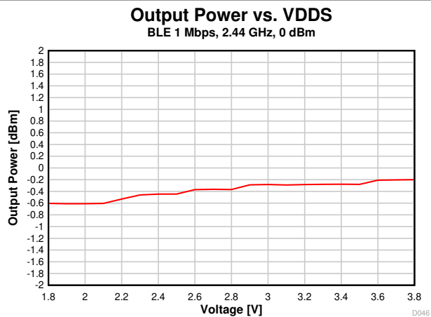
图 8-25. Output Power vs. Supply Voltage (VDD5) (BLE 1 Mbps, 2.44 GHz)
