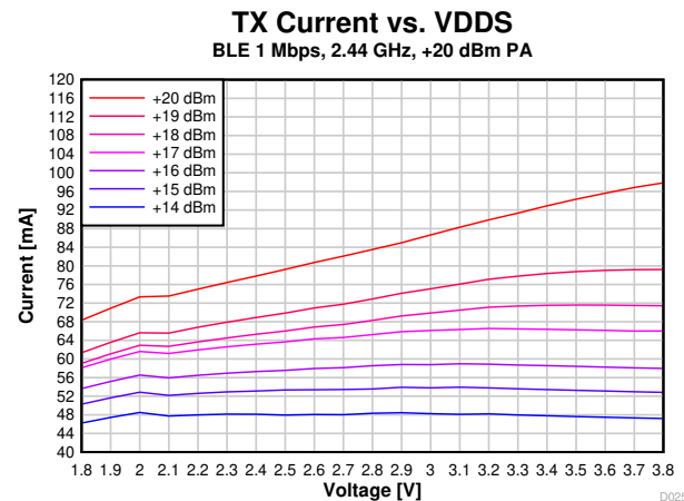
图 8-12. TX Current vs. Supply Voltage (VDD5) (BLE 1 Mbps, 2.44 GHz, +20 dBm PA)
