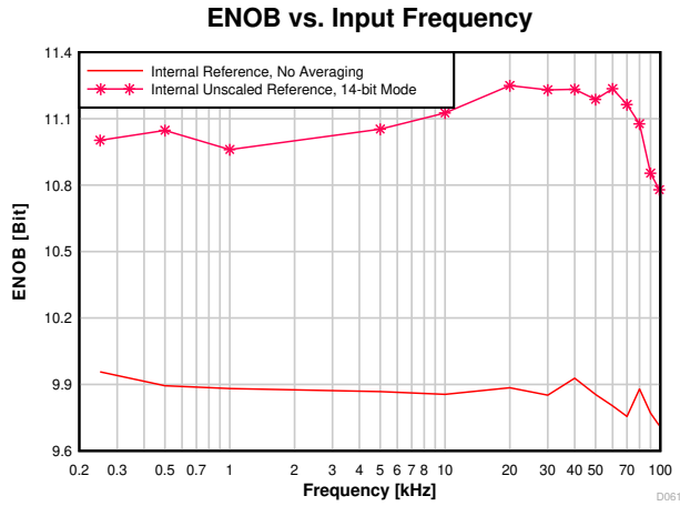
图 8-33. ENOB vs. Input Frequency
