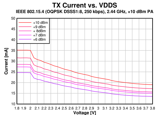
图 8-13. TX Current vs. Supply Voltage (VDD5) (250 kbps, 2.44 GHz, +10 dBm PA)
