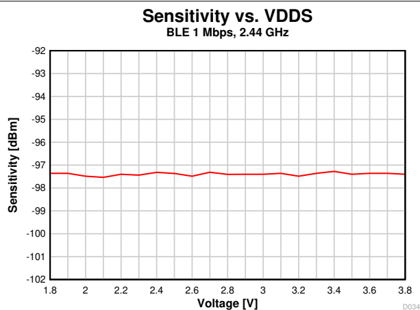
图 8-18. Sensitivity vs. Supply Voltage (VDD) (BLE 1 Mbps, 2.44 GHz)
