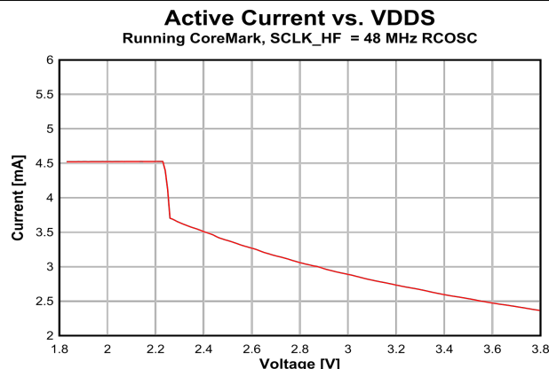
图 8-4. Active Mode (MCU) Current vs. Supply Voltage (VDD)
