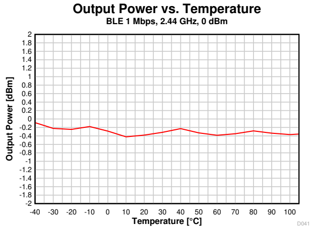
图 8-21. Output Power vs. Temperature (BLE 1 Mbps, 2.44 GHz)
