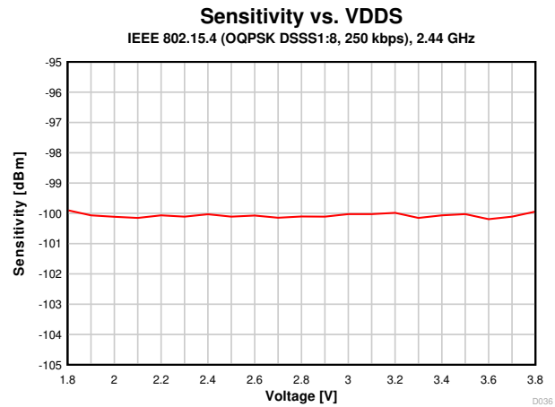
图 8-20. Sensitivity vs. Supply Voltage (VDDS) (250 kbps, 2.44 GHz)
