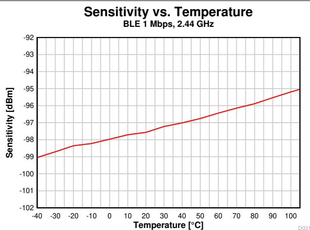
图 8-16. Sensitivity vs. Temperature (BLE 1 Mbps, 2.44 GHz)
