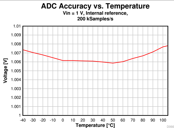
图 8-37. ADC Accuracy vs. Temperature
