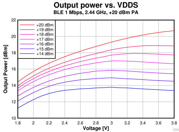
图 8-27. Output Power vs. Supply Voltage (VDD5) (BLE 1 Mbps, 2.44 GHz, +20 dBm PA)
