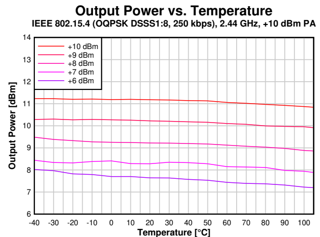
图 8-24. Output Power vs. Temperature (2.44 GHz, +10 dBm PA)
