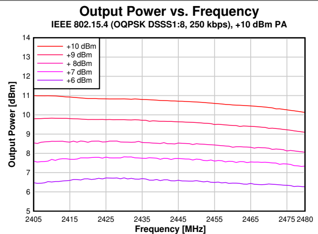
图 8-32. Output Power vs. Frequency (250 kbps, +10 dBm PA)
