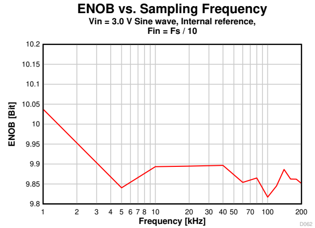
图 8-34. ENOB vs. Sampling Frequency
