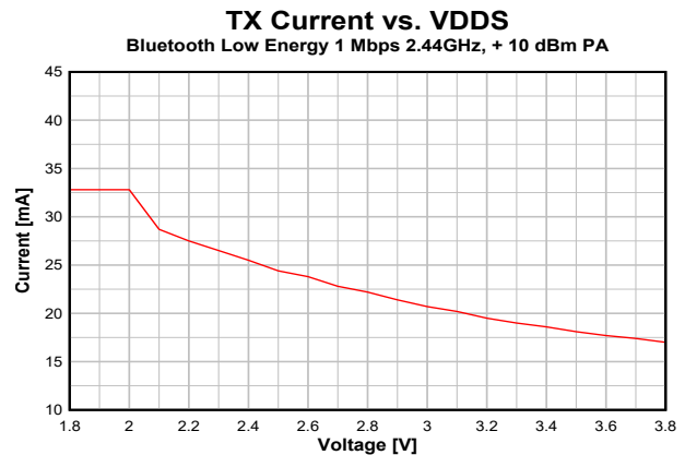
图 8-11. TX Current vs. Supply Voltage (VDD5) (BLE 1 Mbps, 2.44 GHz)
