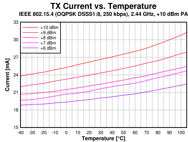
图 8-10. TX Current vs. Temperature (250 kbps, 2.44 GHz, +10 dBm PA)
