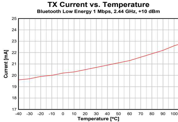
图 8-8. TX Current vs. Temperature (BLE 1 Mbps, 2.44 GHz)
