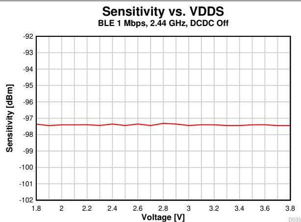
图 8-19. Sensitivity vs. Supply Voltage (VDD) (BLE 1 Mbps, 2.44 GHz, DCDC Off)
