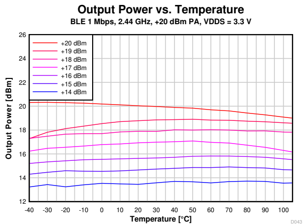
图 8-23. Output Power vs. Temperature (BLE 1 Mbps, 2.44 GHz, +20 dBm PA)
