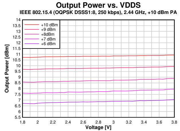
图 8-28. Output Power vs. Supply Voltage (VDD5) (2.44 GHz, +10 dBm PA)
