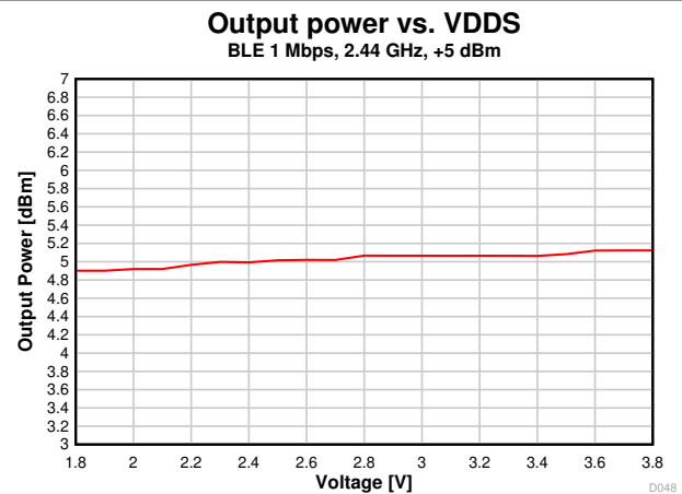
图 8-26. Output Power vs. Supply Voltage (VDD5) (BLE 1 Mbps, 2.44 GHz, +5 dBm)
