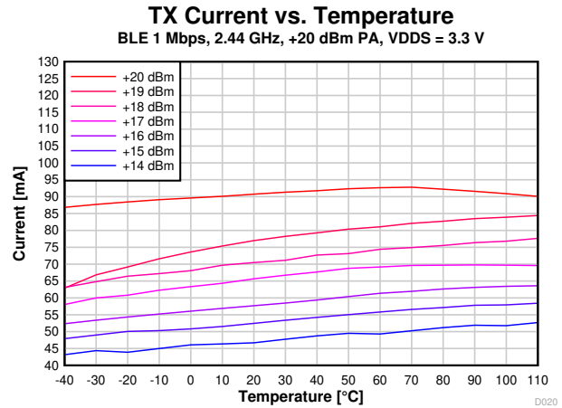
图 8-9. TX Current vs. Temperature (BLE 1 Mbps, 2.44 GHz, VDD5 = 3.3 V)
