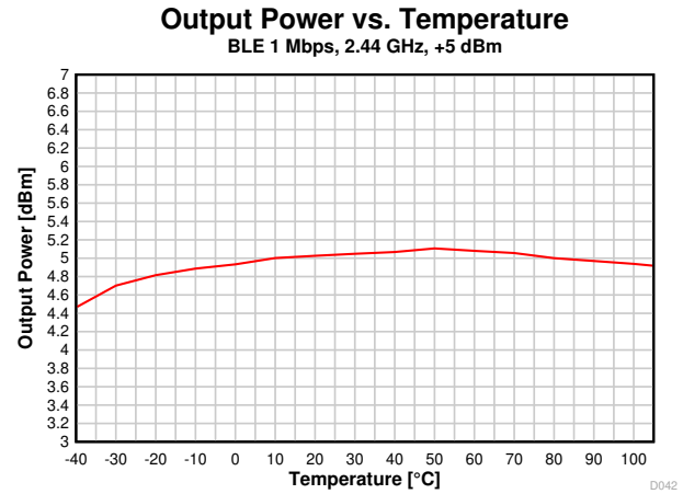
图 8-22. Output Power vs. Temperature (BLE 1 Mbps, 2.44 GHz, +5 dBm)
