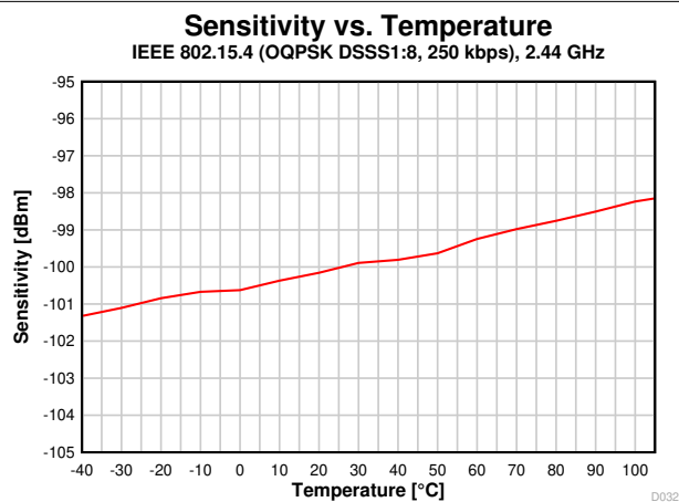
图 8-17. Sensitivity vs. Temperature (250 kbps, 2.44 GHz)
