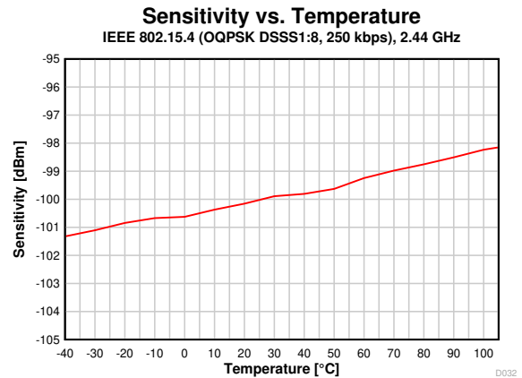
图 7-17. Sensitivity vs. Temperature (IEEE 802.15.4-2006, 250 kbps, OQPSK DSSS 1:8, 2.44GHz)
