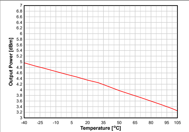
图 8-22. Output Power vs. Temperature (BLE 1 Mbps, 2.44 GHz, +5 dBm)
