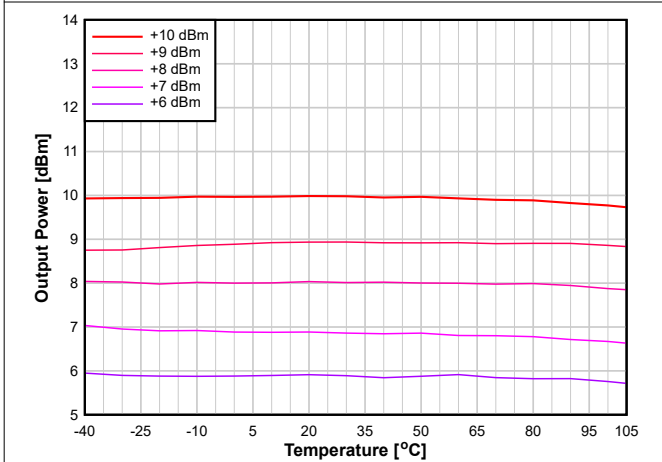
图 8-23. Output Power vs. Temperature (BLE 1 Mbps, 2.44 GHz, +10 dBm)
