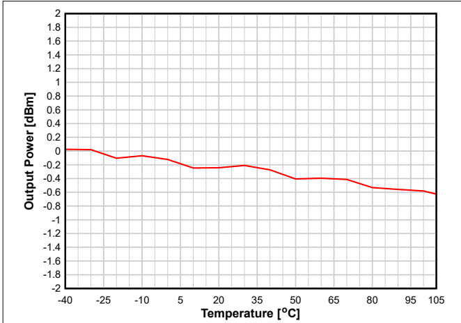
图 8-21. Output Power vs. Temperature (BLE 1 Mbps, 2.44 GHz, 0 dBm)
