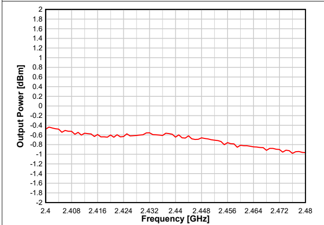
图 8-23. Output Power vs. Frequency (BLE 1 Mbps, 0 dBm)
