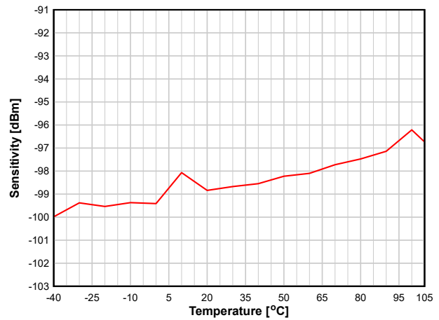
图 8-15. Sensitivity vs. Temperature (250 kbps, 2.44 GHz)
