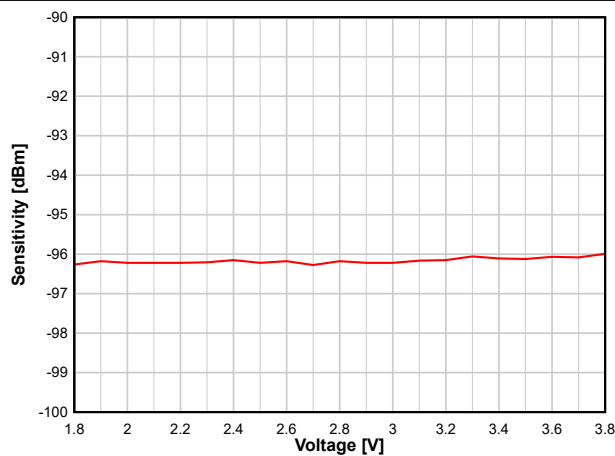
图 8-16. Sensitivity vs. Supply Voltage (VDD) (BLE 1 Mbps, 2.44 GHz)
