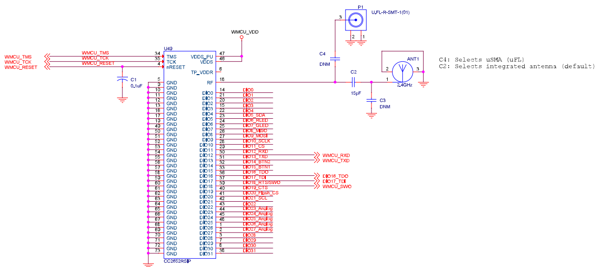
图 10-1. CC2652RSIP Typical Application Schematic
