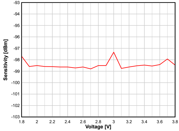
图 8-18. Sensitivity vs. Supply Voltage (VDD5) (250 kbps, 2.44 GHz)
