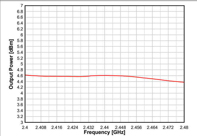
图 8-24. Output Power vs. Frequency (BLE 1 Mbps, +5 dBm)
