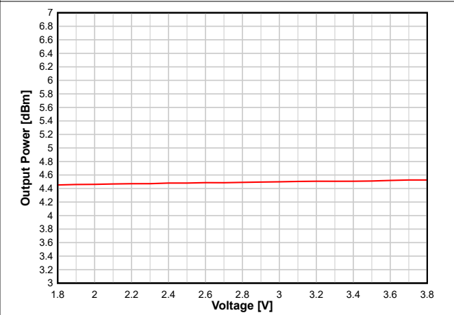
图 8-22. Output Power vs. Supply Voltage (VDDS) (BLE 1 Mbps, 2.44 GHz, +5 dBm)
