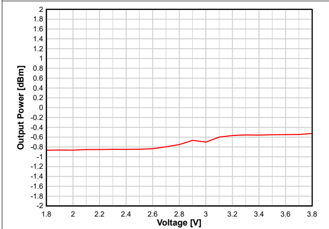
图 8-21. Output Power vs. Supply Voltage (VDDS) (BLE 1 Mbps, 2.44 GHz, 0 dBm)
