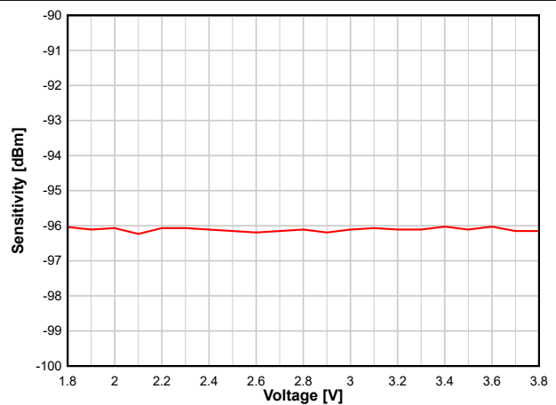
图 8-17. Sensitivity vs. Supply Voltage (VDD) (BLE 1 Mbps, 2.44 GHz, DCDC Off)
