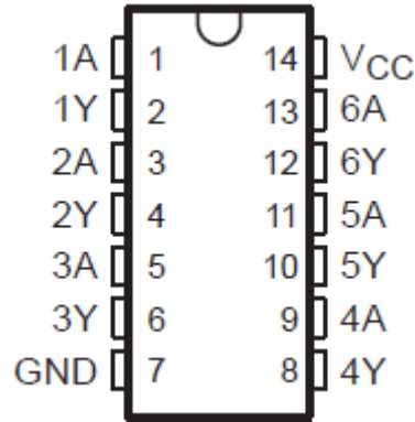
图 3-1. N or D Package, 14-Pin PDIP or SOIC Top View
