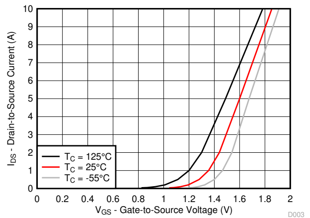
Figure 5-3. Transfer Characteristics
