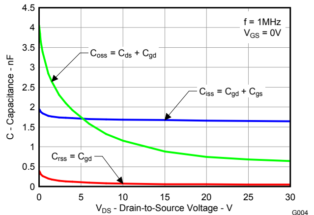
Figure 5. Capacitance
