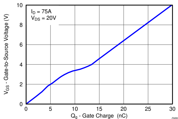
栅极电荷
