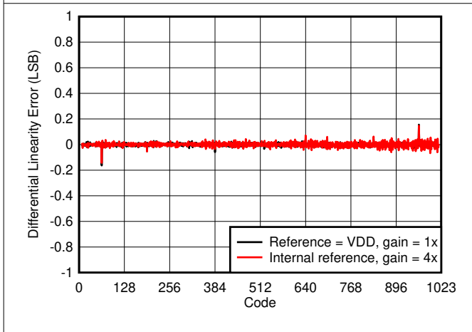
图 6-4. Differential Linearity Error vs Digital Input Code
