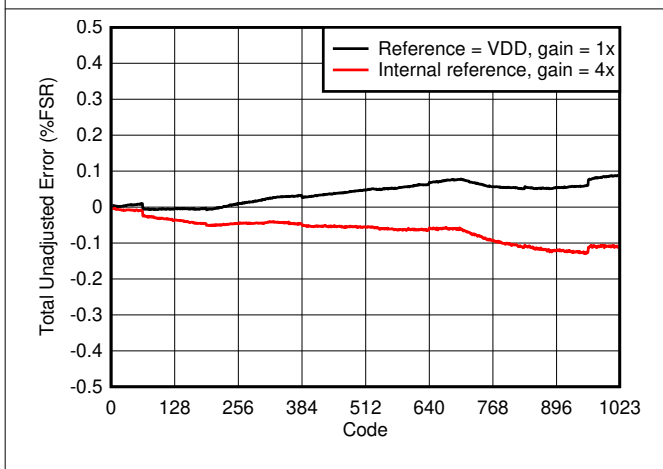
图 6-6. Total Unadjusted Error vs Digital Input Code
