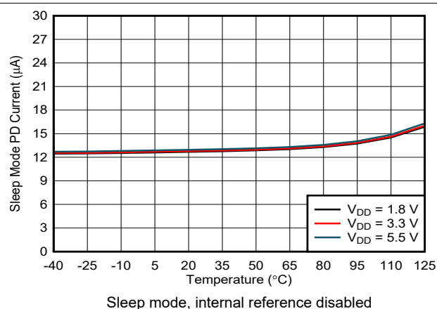
图 6-62. Power-Down Current vs Temperature
