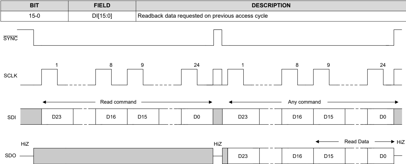
图 7-15. SPI Read Cycle
