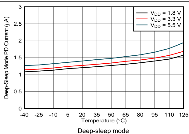
图 6-63. Power-Down Current vs Temperature
