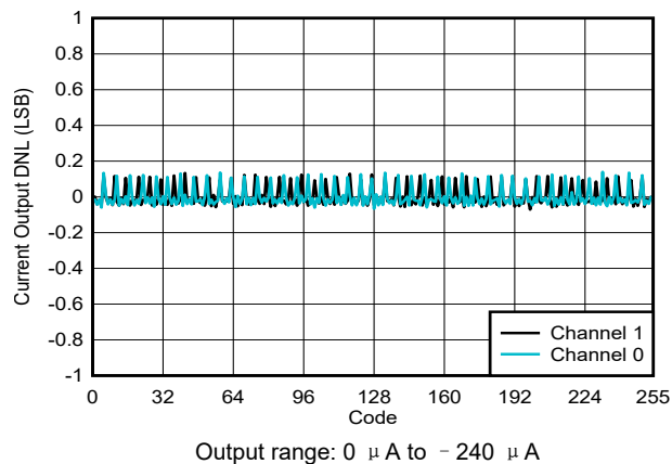
图 6-37. Current Output DNL vs Digital Input Code
