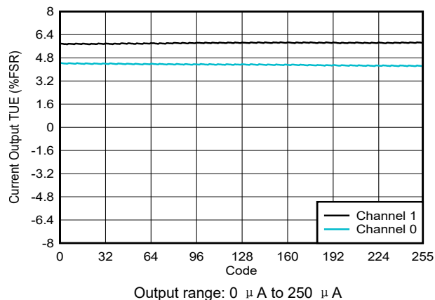
图 6-41. Current Output TUE vs Digital Input Code
