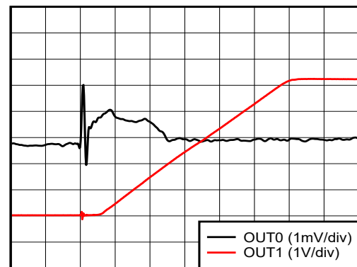
Time (500ns/div)
