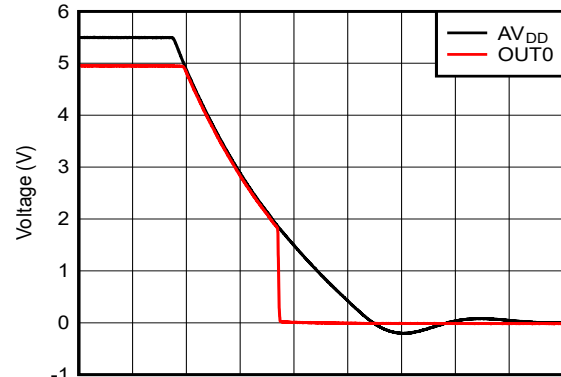
Time (100µs/div)
