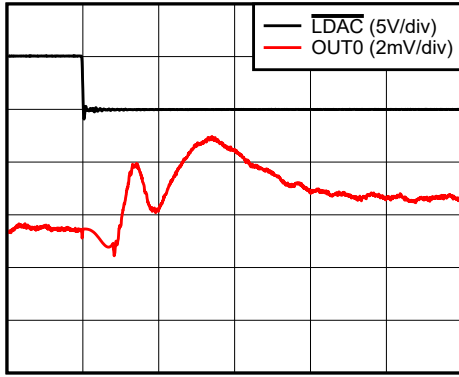
Time (250ns/div)
