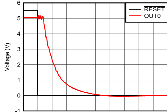
Time (50ns/div)
