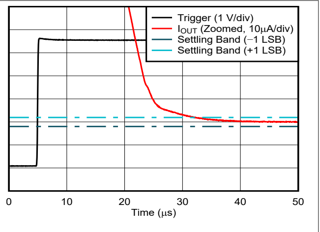
图 6-49. Current Output Setting Time, Falling Edge
