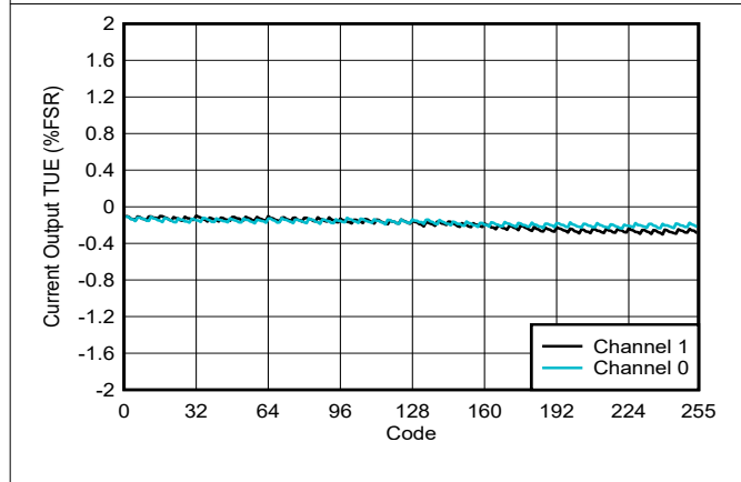
图 6-40. Current Output TUE vs Digital Input Code
