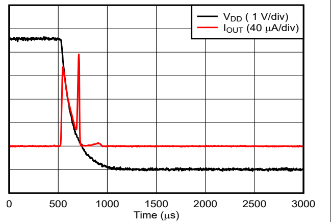
图 6-49. Current Output Setting Time, Falling Edge
