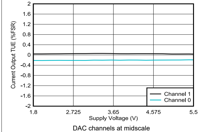
图 6-44. Current Output TUE vs Supply Voltage
