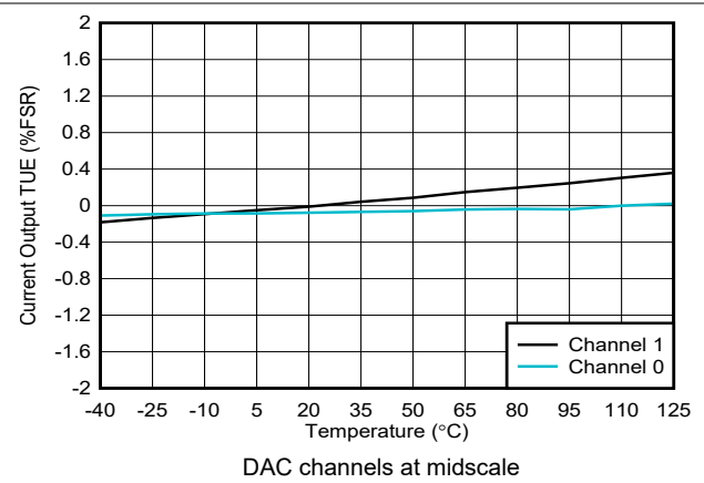
图 6-43. Current Output TUE vs Temperature
