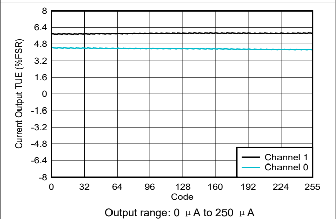
图 6-41. Current Output TUE vs Digital Input Code
