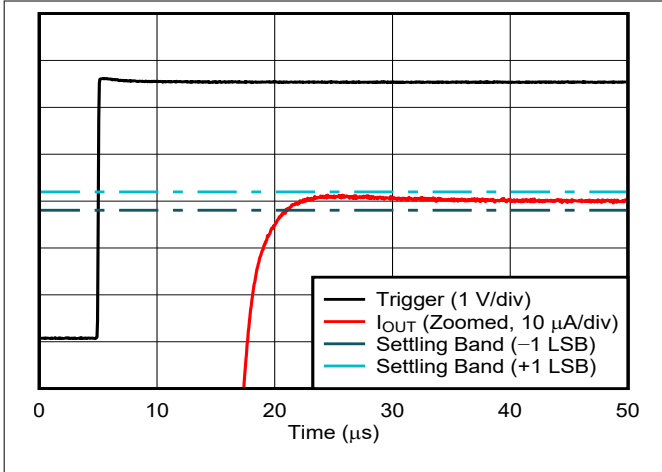
图 6-48. Current Output Setting Time, Rising Edge
