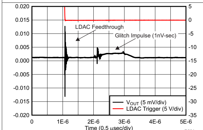
DAC code transition from 8000h to 7FFFh
