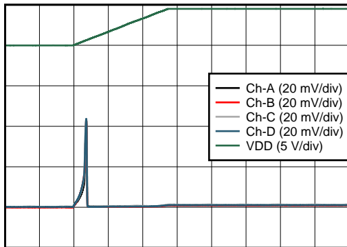
Time (0.2 ms/div)
