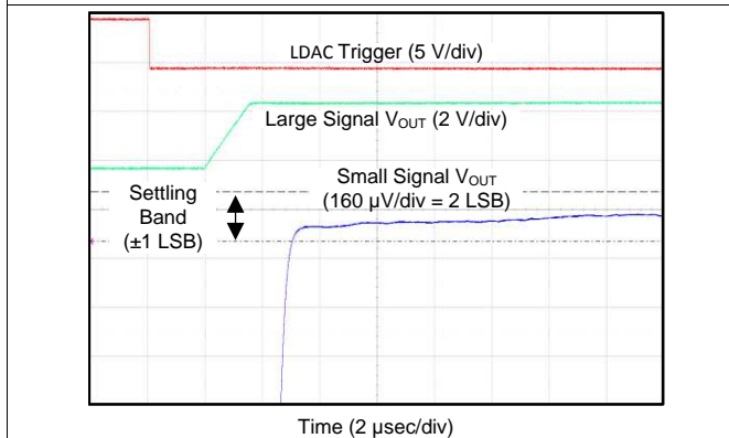
From code 512d to 65024d, Typical channel shown
