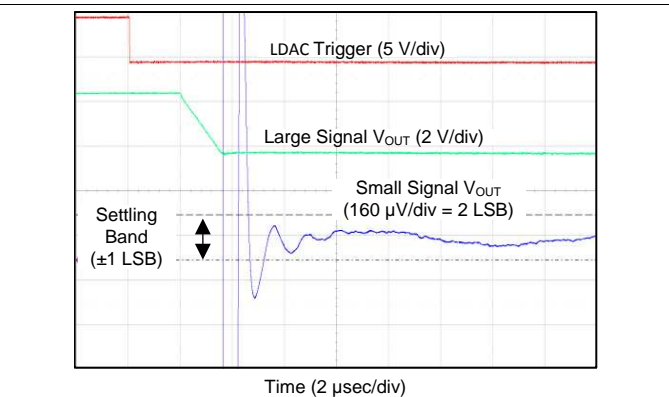
From code 65024d to 512d, Typical channel shown
