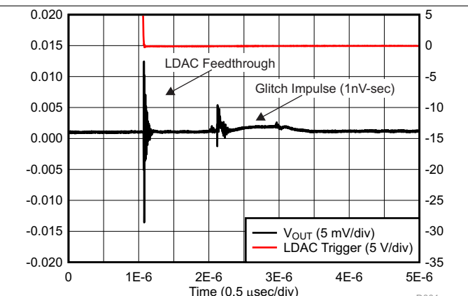
DAC code transition from 7FFFh to 8000h
