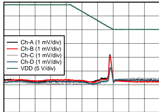
Time (2 ms/div)
