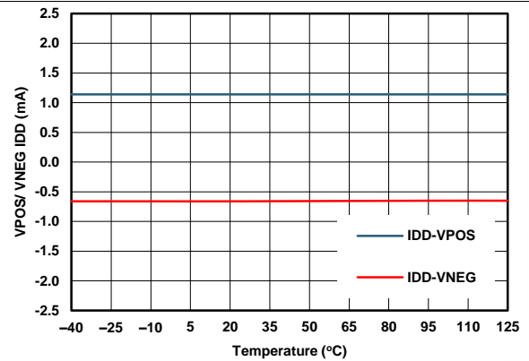
图 22. IOOUT Power Supply Current vs Temperature
