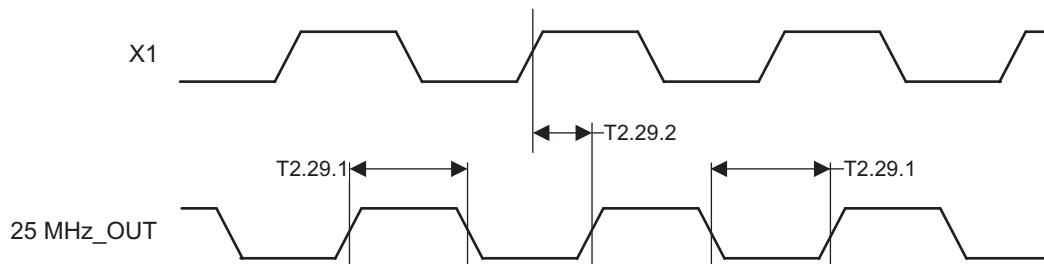
图 4-30. 25MHz_OUT Timing
