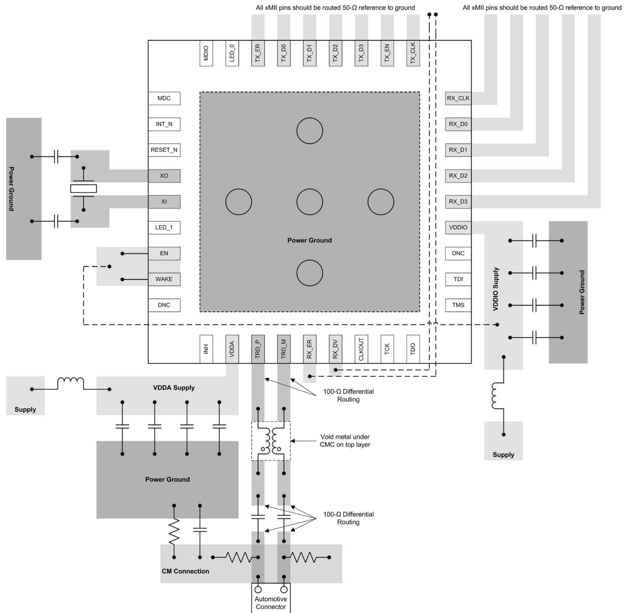
图 8-14. DP83TC811-Q1 MII / RMII / RGMII Layout Recommendation
