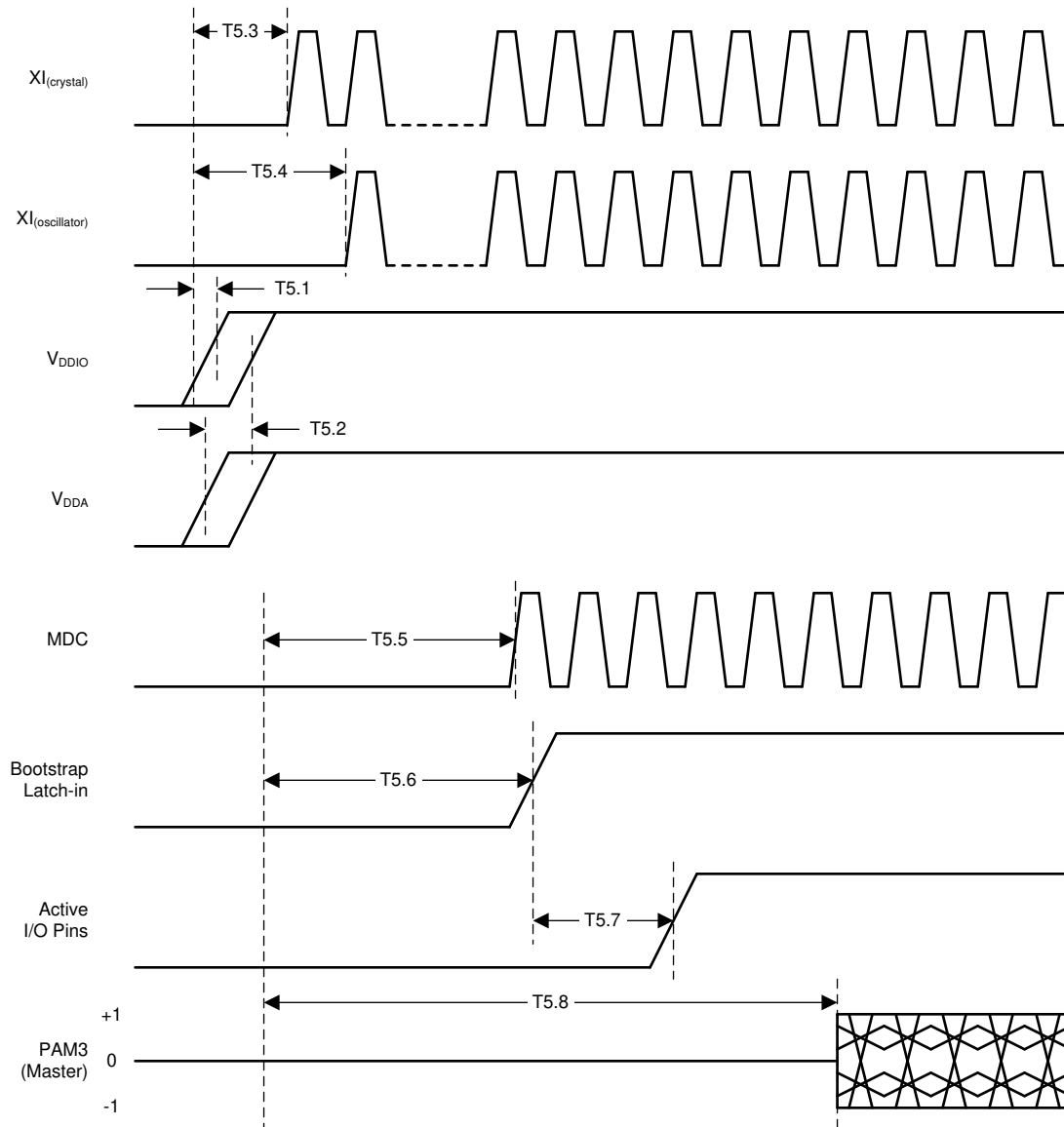
图 6-9. Power-Up Timing
