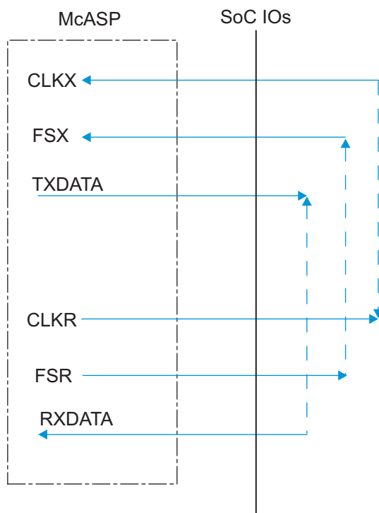
图 7-45. McASP1-8 CIOFIO – ASYNC Mode
