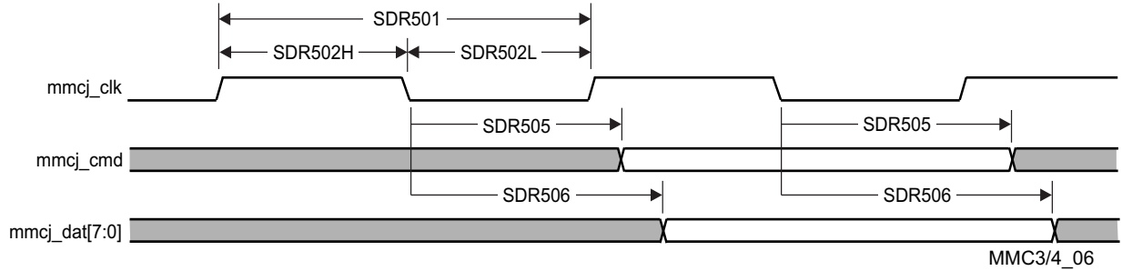
Figure 5-108. MMC/SD/SDIOj in - High-Speed SDR50 - Transmitter Mode
