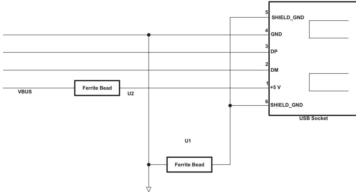
图 7-32. USB Connector
