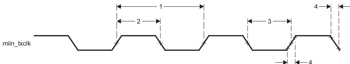
Figure 5-69. Clock Timing (GMAC Transmit) - MII n Operation
