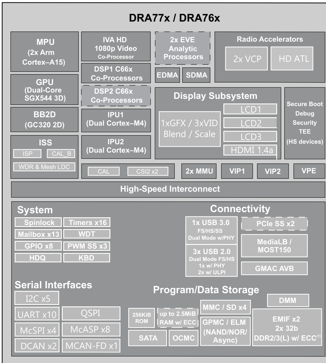
图 6-1. DRA77x, DRA76x Block Diagram
