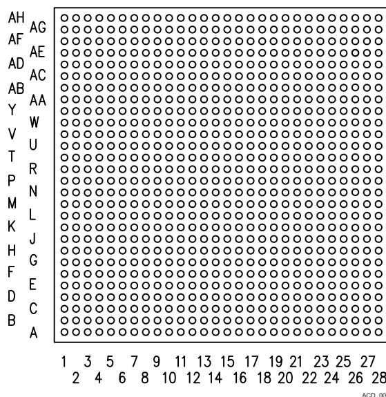
图 4-1. ACD S-PBGA-N784 Package (Bottom View)
