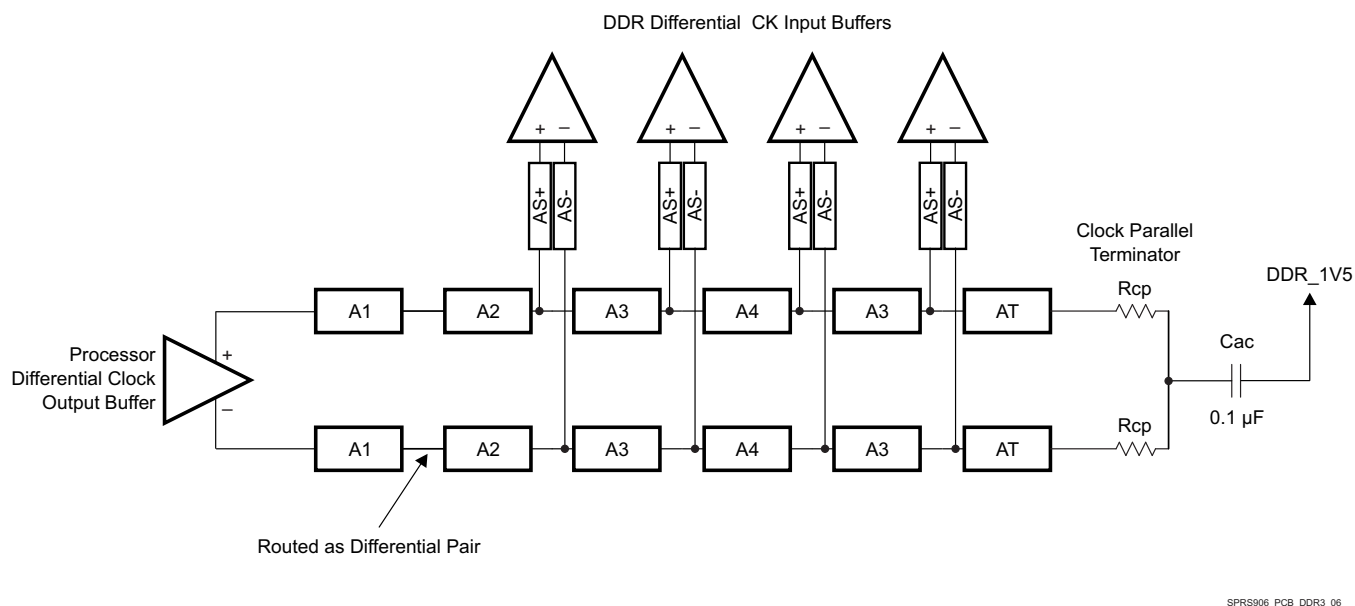
图 7-59. CK Topology for Four x8 DDR3 Devices
