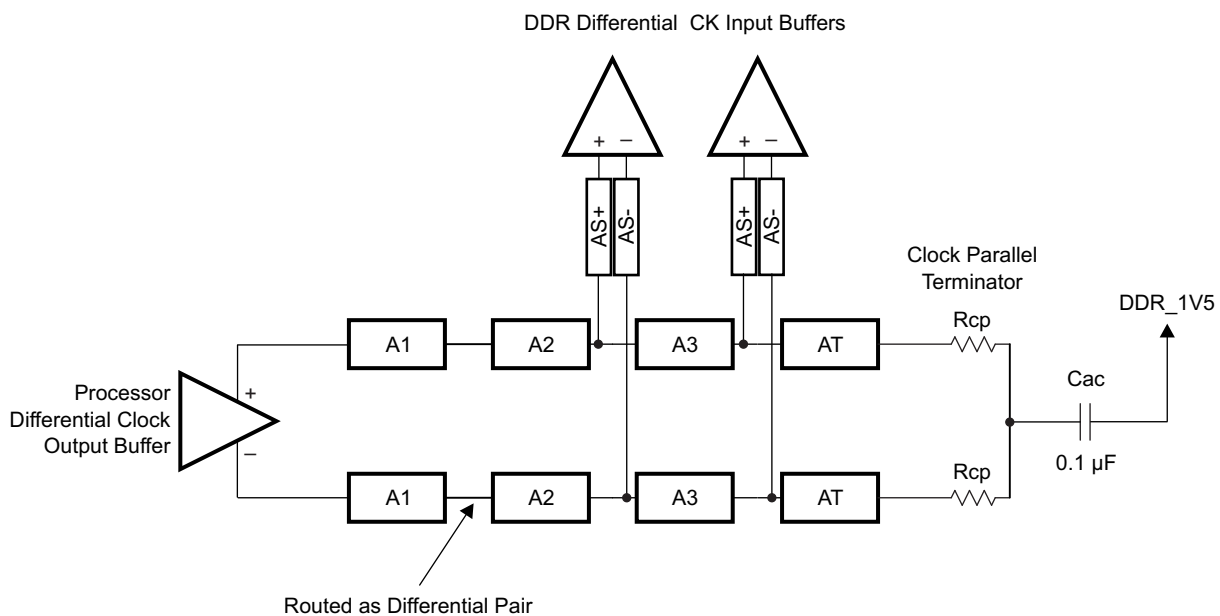
SPRS906_PCB_DDR3_12
