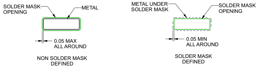
SOLDER MASK DETAILS PADS 1-20
