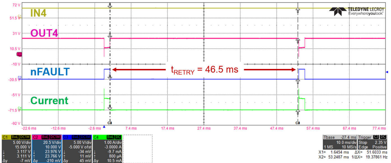
图 7-3. t_{\text{RETRY}} = 46.5\text{ms} , 启用截止延迟 (COD), R_{\text{COD}} = 180\text{k}\Omega , 12V, 12 \Omega 1mH 负载, VCLAMP 短接至 VM
