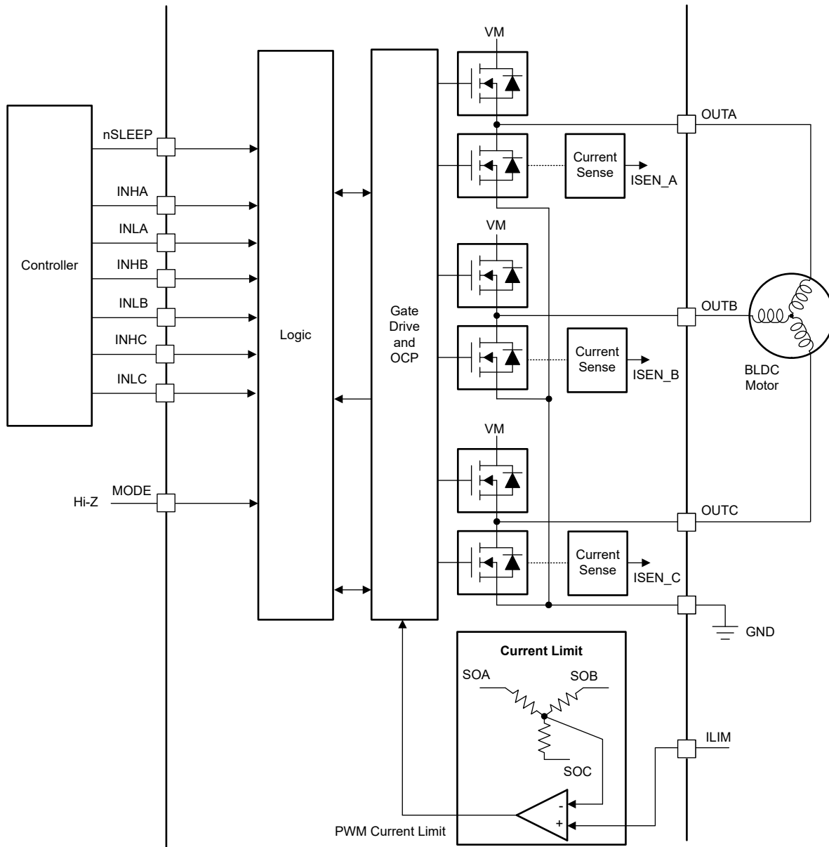
图 8-5. 6x PWM Mode with Current Limit
