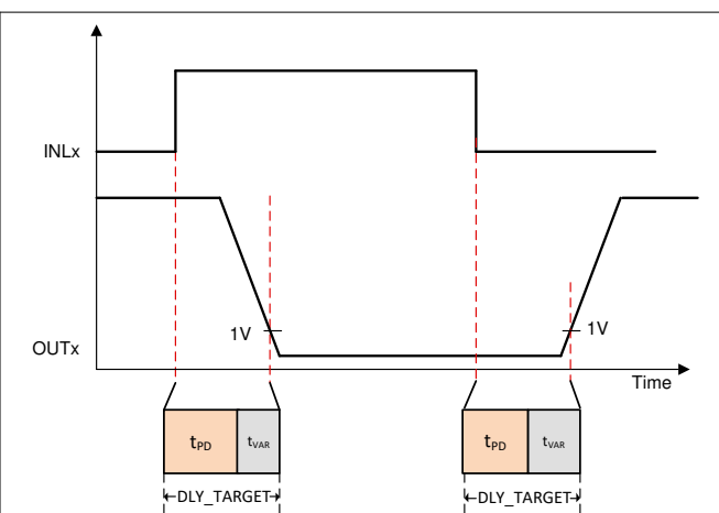
图 8-22. Delay Compensation with current flowing into the phase
