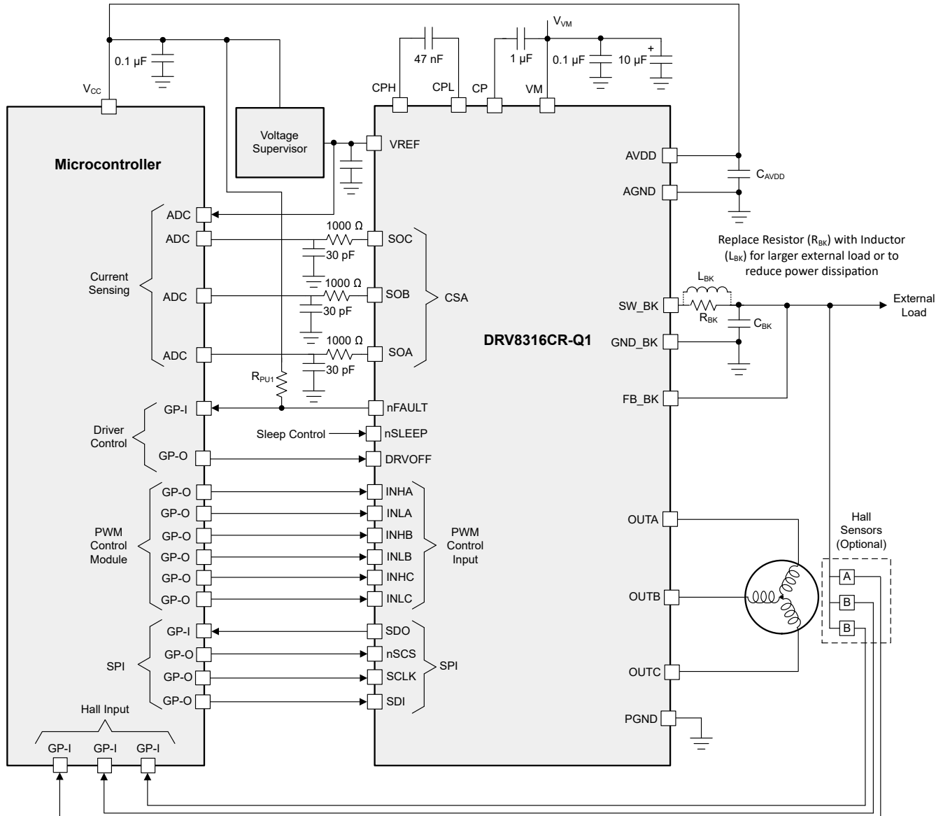
图 9-1. Primary Application Schematic
