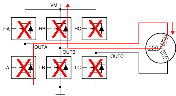
图 8-39. Coast State
