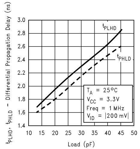
图 6-10. Differential Propagation Delay vs Load
