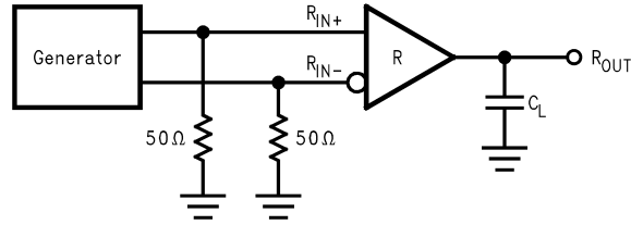
图 7-1. Receiver Propagation Delay and Transition Time Test Circuit
