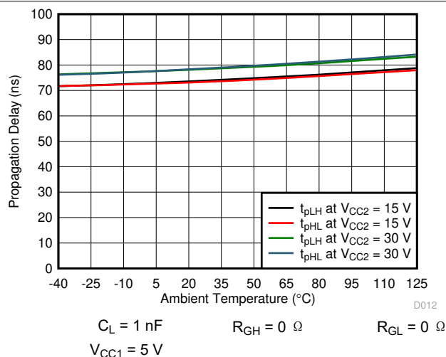
图 7-25. Propagation Delay vs Temperature
