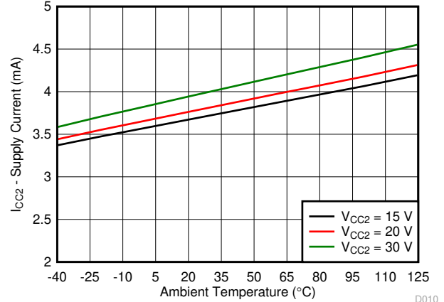
图 7-22. I_{CC2} Supply Current vs Temperature
