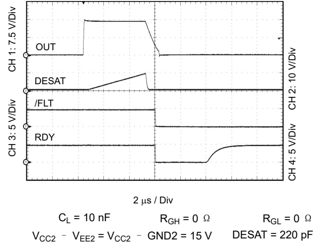
图 7-16. Output Transient Waveform DESAT, RDY, and FLT
