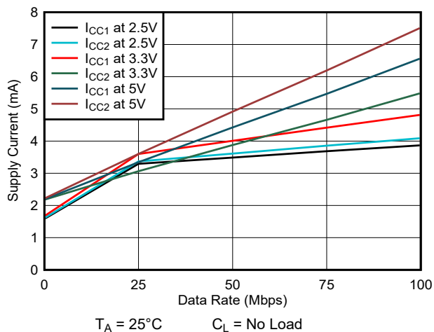
图 5-6. ISO7730-Q1 Supply Current vs Data Rate (With No Load)
