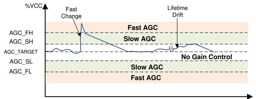
图 8-3. AGC Regulation Bands
