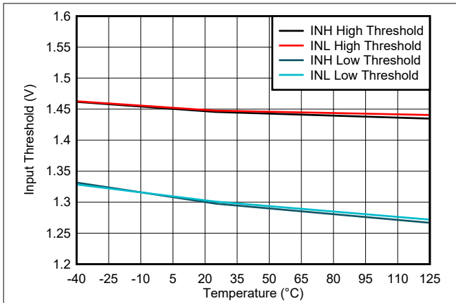
图 6-14. Input Voltage Thresholds vs Temperature
