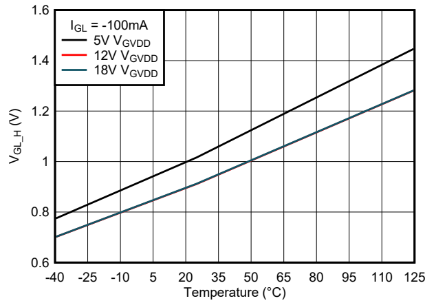
图 6-8. GL Output High Voltage vs Temperature
