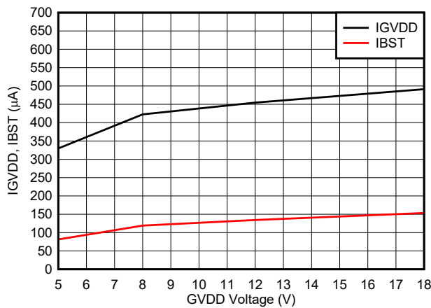
图 6-6. Quiescent Currents vs Supply Voltage
