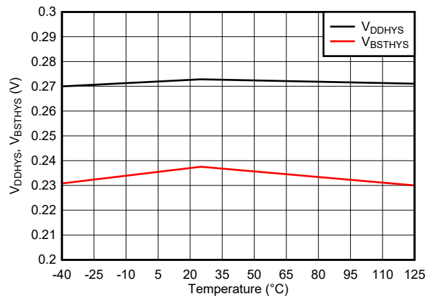
图 6-13. GVDD and BST UVLO Hysteresis vs Temperature
