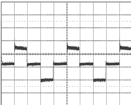
Conditions: Input Voltage = 24 VDC Output Current = 5 A Trace: Q1 drain-to-source voltage, V/div = 20 V Horizontal Resolution = 2 \mu s/div
