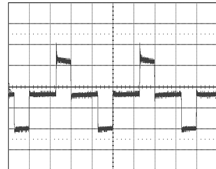
Conditions: Input Voltage = 32 VDC Output Current = 5 A Trace: Q1 drain to source voltage, V/div = 20 V Horizontal Resolution = 2 \mu s/div
