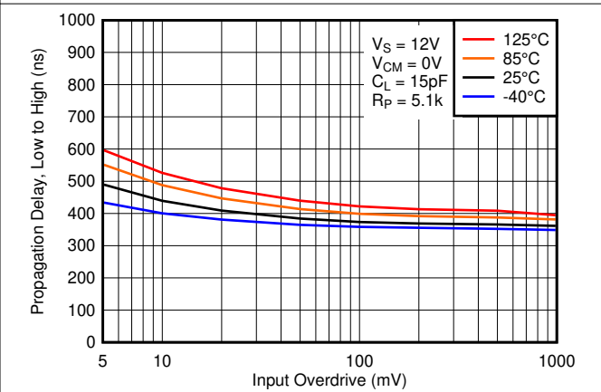
图 7-28. Low to High Propagation Delay vs. Input Overdrive Voltage, 12V
