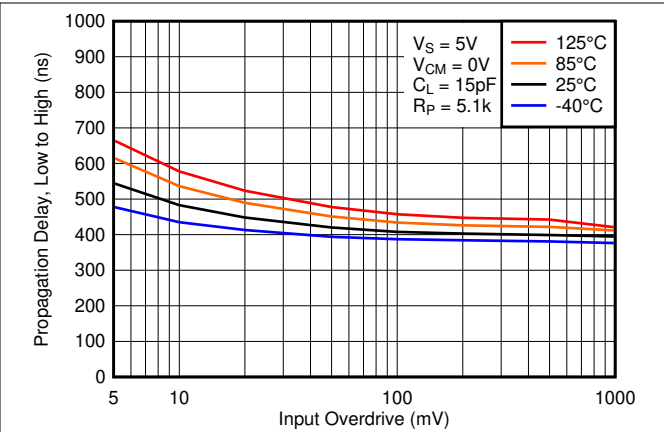
图 7-26. Low to High Propagation Delay vs. Input Overdrive Voltage, 5V
