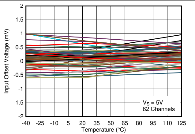
图 7-8. Input Offset Voltage vs. Temperature at 5V
