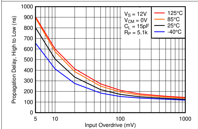
图 7-27. High to Low Propagation Delay vs. Input Overdrive Voltage, 12V
