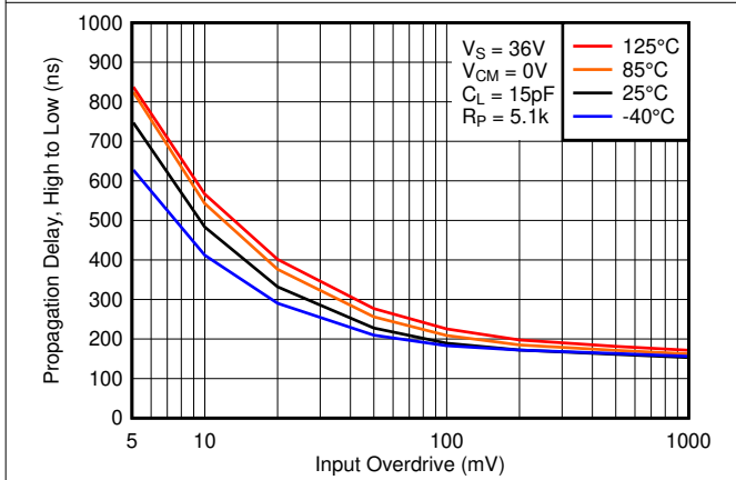
图 7-29. High to Low Propagation Delay vs. Input Overdrive Voltage, 36V
