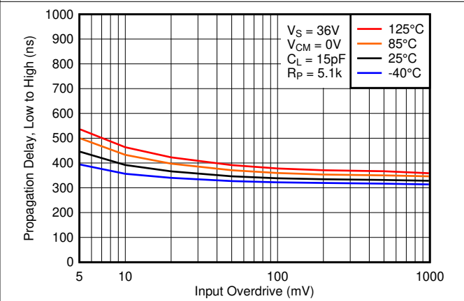
图 7-30. Low to High Propagation Delay vs. Input Overdrive Voltage, 36V
