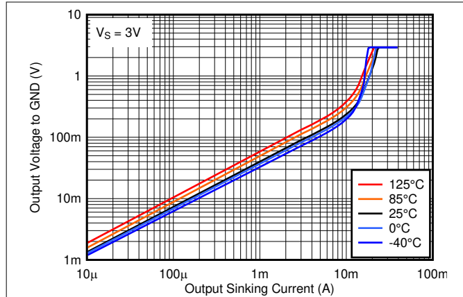
图 7-19. Output Low Voltage vs. Output Sinking Current at 3V
