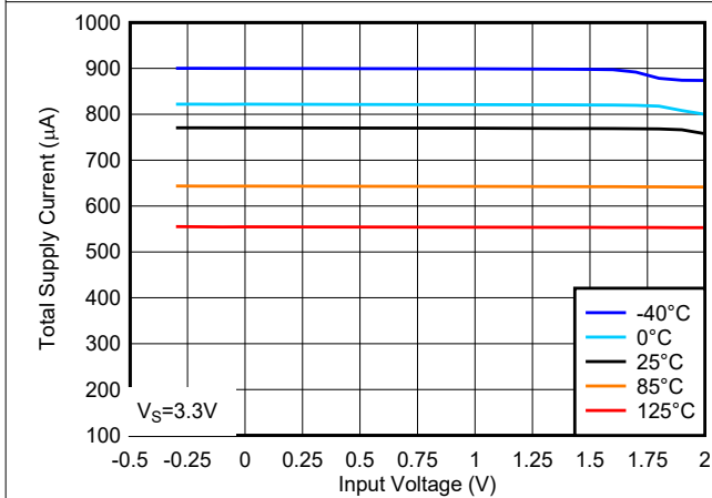
图 7-3. Total Supply Current vs. Input Voltage at 3.3V
