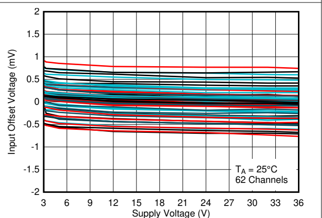
图 7-12. Input Offset Voltage vs. Supply Voltage at 25^\circ\text{C}
