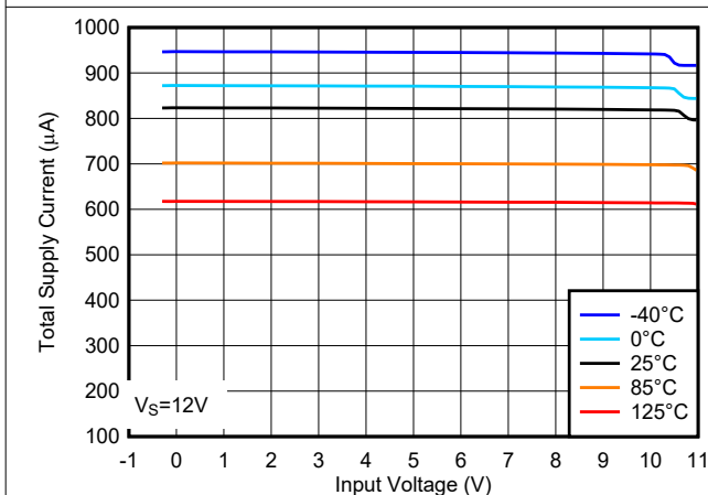
图 7-5. Total Supply Current vs. Input Voltage at 12V
