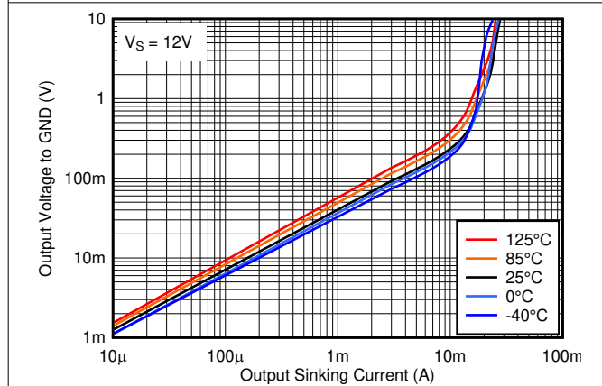
图 7-21. Output Low Voltage vs. Output Sinking Current at 12V
