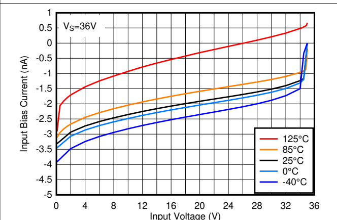
图 7-18. Input Bias Current vs. Input Voltage at 36V
