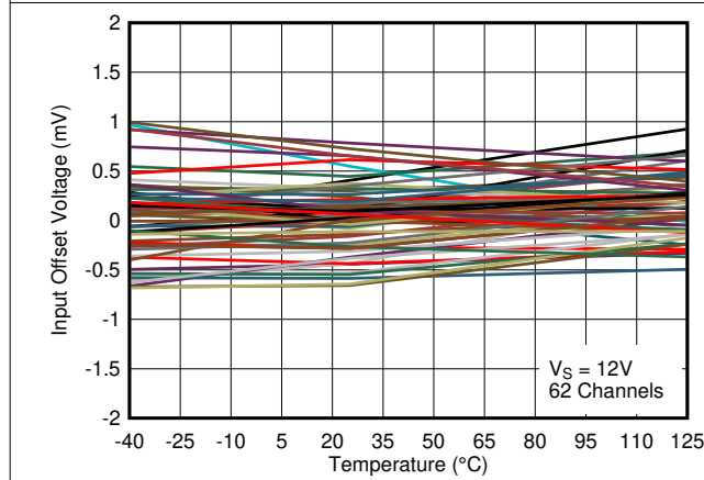
图 7-9. Input Offset Voltage vs. Temperature at 12V
