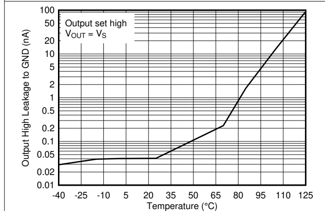
图 7-23. Output High Leakage Current vs. Temperature at 5V
