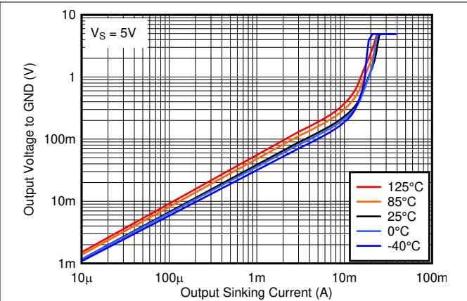
图 7-20. Output Low Voltage vs. Output Sinking Current at 5V
