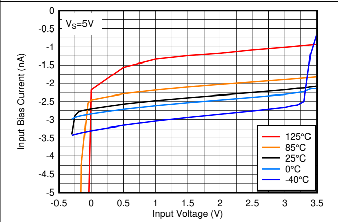
图 7-16. Input Bias Current vs. Input Voltage at 5V
