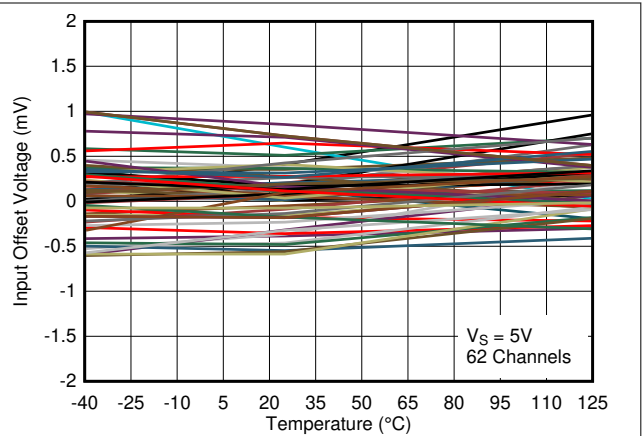
图 7-8. Input Offset Voltage vs. Temperature at 5V
