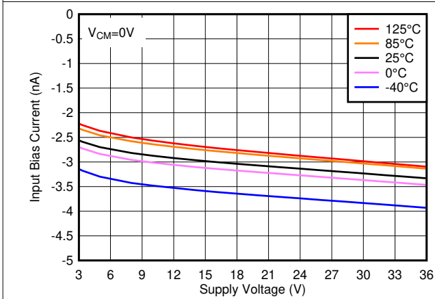
图 7-15. Input Bias Current vs. Supply Voltage
