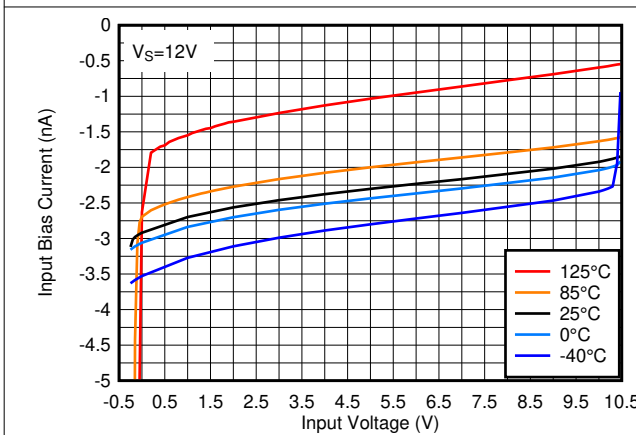
图 7-17. Input Bias Current vs. Input Voltage at 12V
