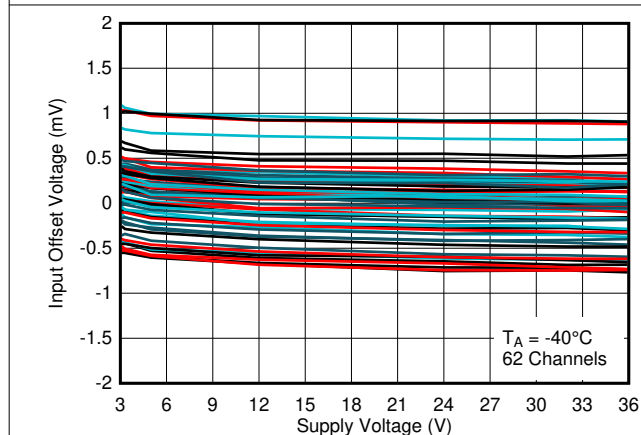
图 7-11. Input Offset Voltage vs. Supply Voltage at -40^\circ\text{C}
