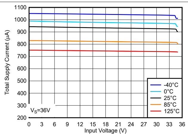
图 7-6. Total Supply Current vs. Input Voltage at 36V
