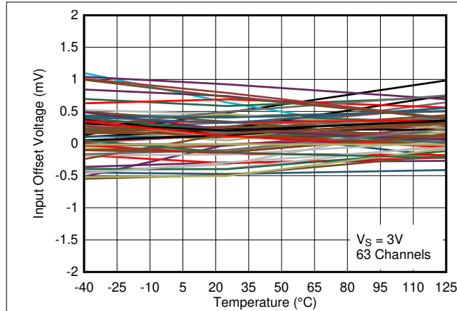
图 7-7. Input Offset Voltage vs. Temperature at 3V
