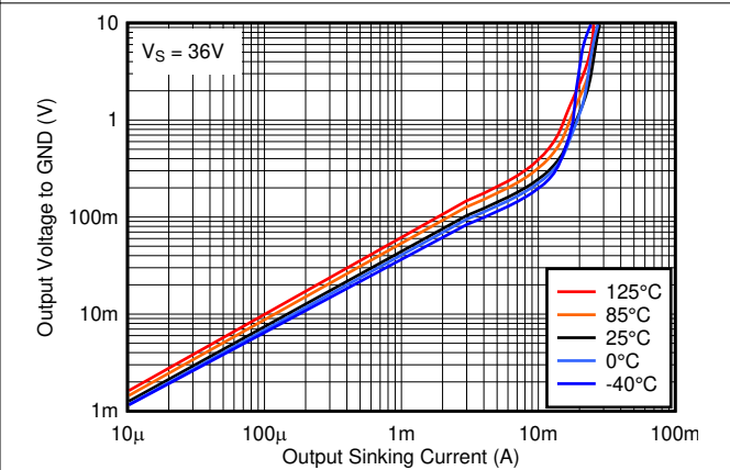
图 7-22. Output Low Voltage vs. Output Sinking Current at 36V
