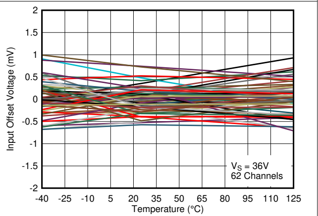
图 7-10. Input Offset Voltage vs. Temperature at 36V
