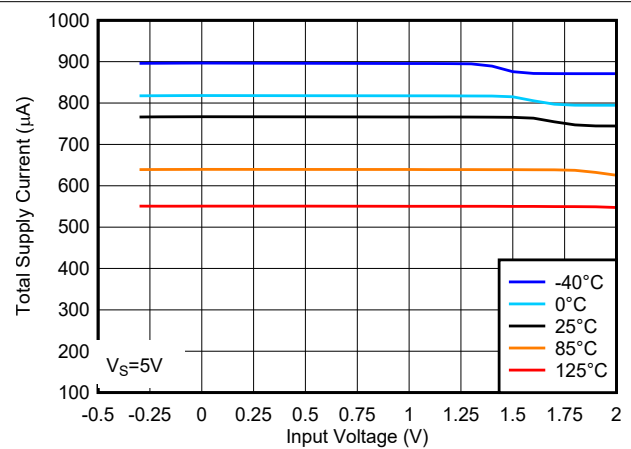
图 7-4. Total Supply Current vs. Input Voltage at 5V
