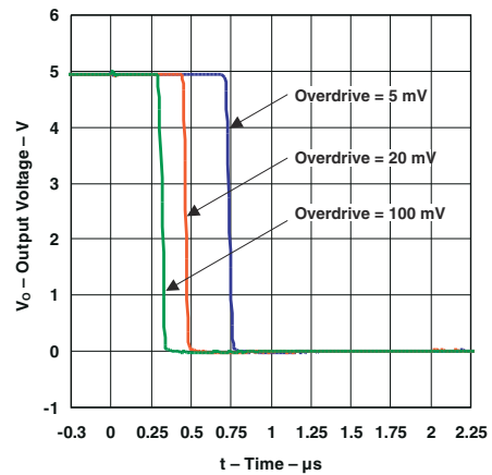
图 7-36. Response Time for Various Overdrives Negative Transition
