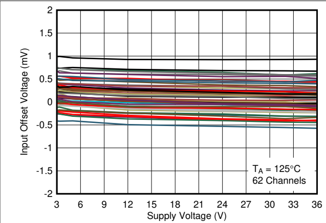
图 3-20. Input Offset Voltage vs. Supply Voltage at 125°C
