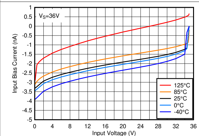
图 3-24. Input Bias Current vs. Input Voltage at 36V
