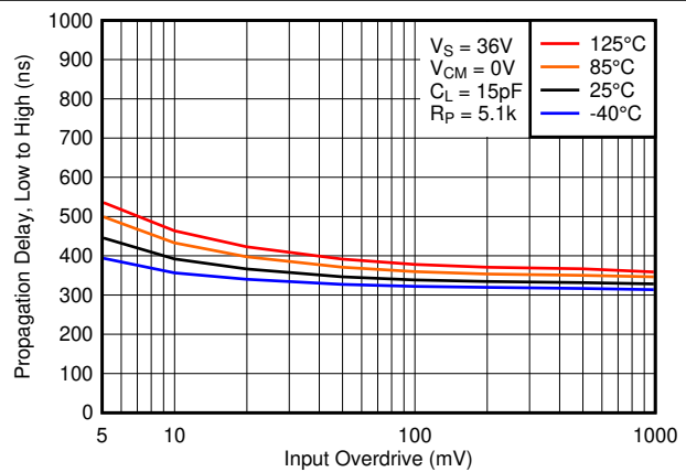
图 6-30. Low to High Propagation Delay vs. Input Overdrive Voltage, 36V
