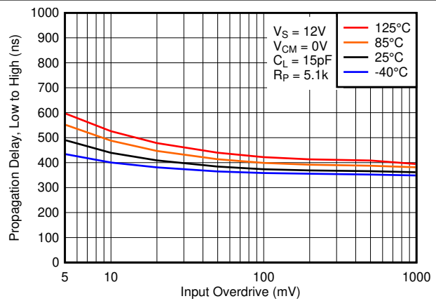
图 6-28. Low to High Propagation Delay vs. Input Overdrive Voltage, 12V
