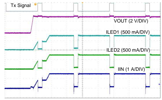
Figure 48. Start-Up
